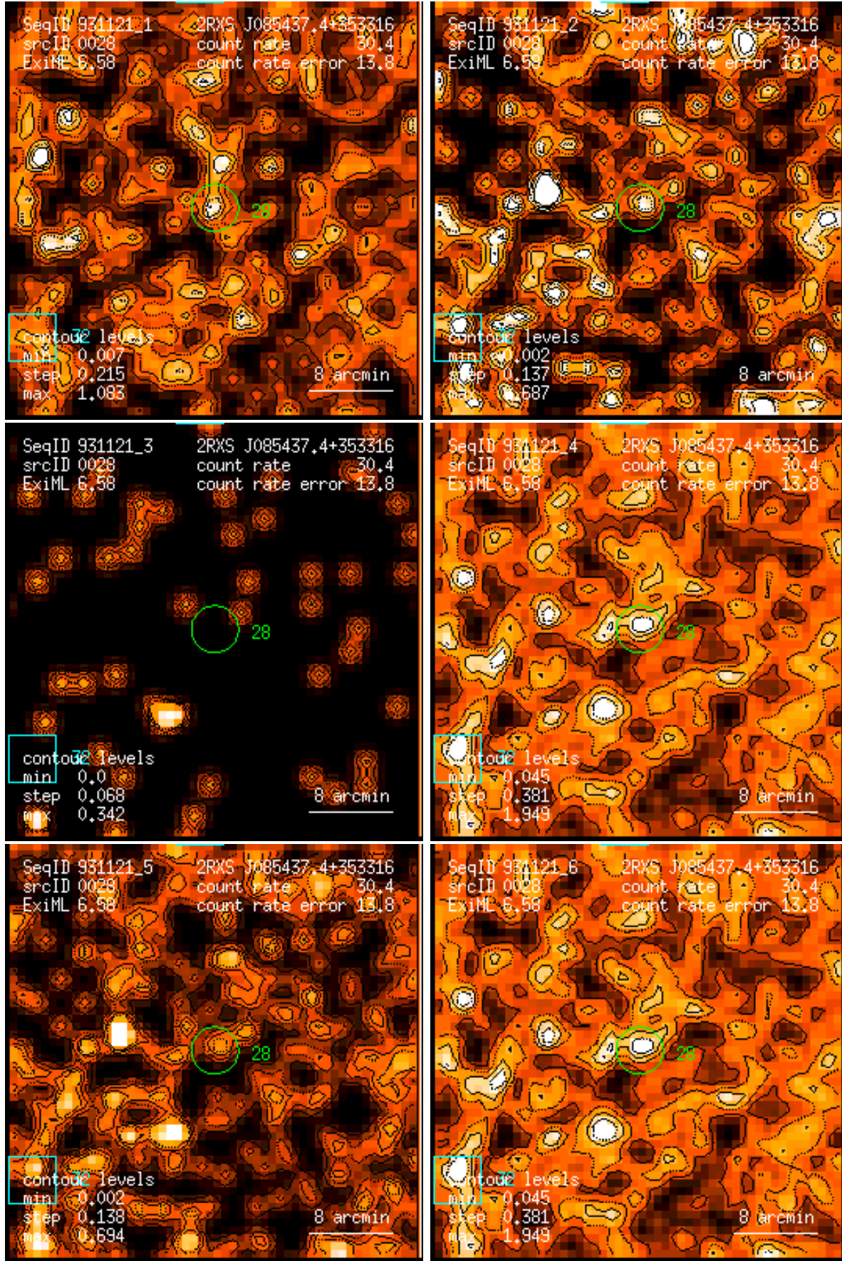
Figure 28: RASS 931121: detection 0028: band rate images, Gaussian filter: (1) PSPC channels 11 – 41, (2) 52 – 90, (3) 91 – 201, (4) 11 – 235, (5) 52 – 201, (6) 11 – 201. Broad band rates in counts/ks. Band rate contour levels in counts/ks/arcmin 2 .
