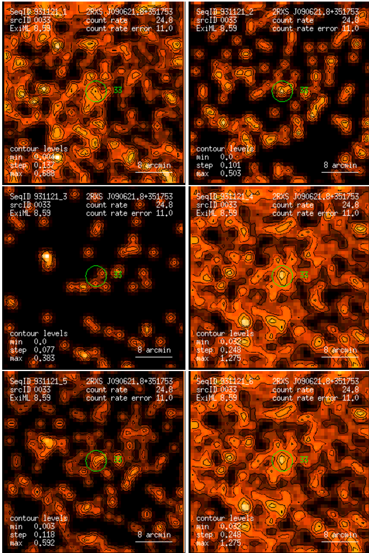
Figure 33: RASS 931121: detection 0033: band rate images, Gaussian filter: (1) PSPC channels 11 – 41, (2) 52 – 90, (3) 91 – 201, (4) 11 – 235, (5) 52 – 201, (6) 11 – 201. Broad band rates in counts/ks. Band rate contour levels in counts/ks/arcmin 2 .
