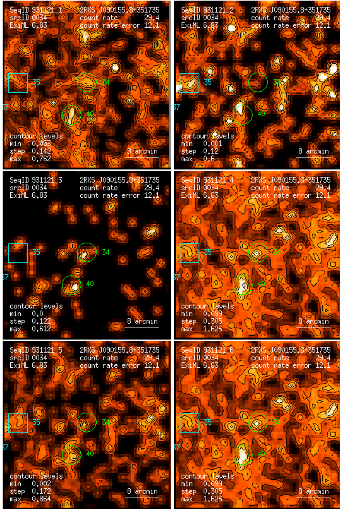
Figure 34: RASS 931121: detection 0034: band rate images, Gaussian filter: (1) PSPC channels 11 – 41, (2) 52 – 90, (3) 91 – 201, (4) 11 – 235, (5) 52 – 201, (6) 11 – 201. Broad band rates in counts/ks. Band rate contour levels in counts/ks/arcmin 2 .
