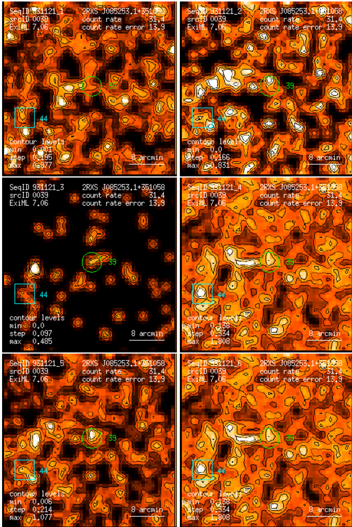
Figure 39: RASS 931121: detection 0039: band rate images, Gaussian filter: (1) PSPC channels 11 – 41, (2) 52 – 90, (3) 91 – 201, (4) 11 – 235, (5) 52 – 201, (6) 11 – 201. Broad band rates in counts/ks. Band rate contour levels in counts/ks/arcmin 2 .
