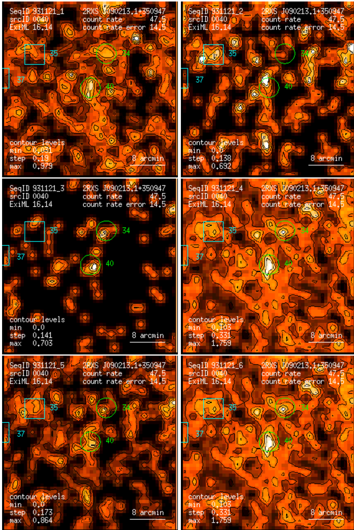
Figure 40: RASS 931121: detection 0040: band rate images, Gaussian filter: (1) PSPC channels 11 – 41, (2) 52 – 90, (3) 91 – 201, (4) 11 – 235, (5) 52 – 201, (6) 11 – 201. Broad band rates in counts/ks. Band rate contour levels in counts/ks/arcmin 2 .
