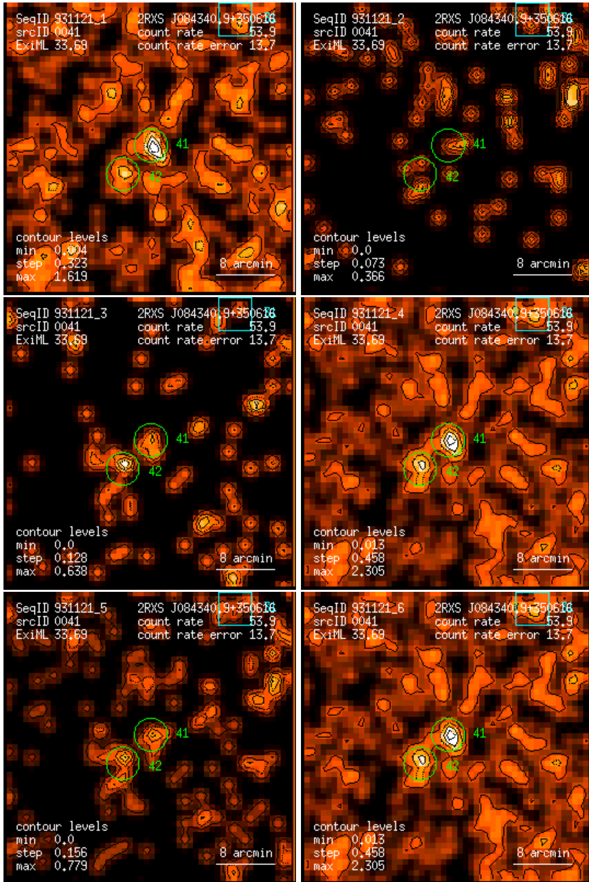
Figure 41: RASS 931121: detection 0041: band rate images, Gaussian filter: (1) PSPC channels 11 – 41, (2) 52 – 90, (3) 91 – 201, (4) 11 – 235, (5) 52 – 201, (6) 11 – 201. Broad band rates in counts/ks. Band rate contour levels in counts/ks/arcmin 2 .
