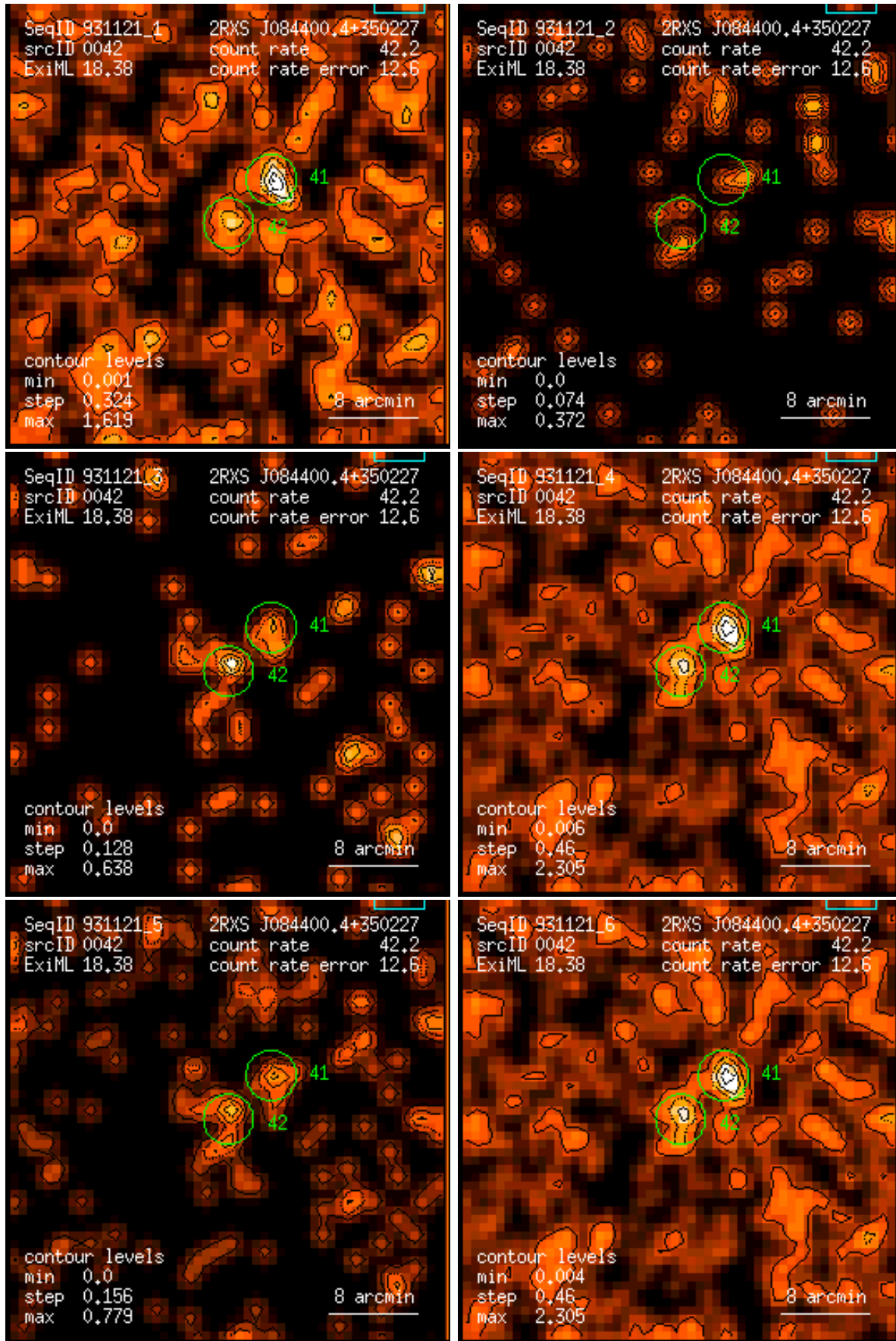
Figure 42: RASS 931121: detection 0042: band rate images, Gaussian filter: (1) PSPC channels 11 – 41, (2) 52 – 90, (3) 91 – 201, (4) 11 – 235, (5) 52 – 201, (6) 11 – 201. Broad band rates in counts/ks. Band rate contour levels in counts/ks/arcmin 2 .
