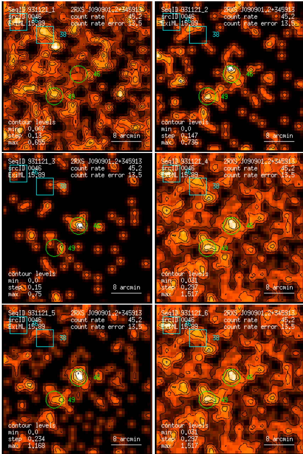
Figure 46: RASS 931121: detection 0046: band rate images, Gaussian filter: (1) PSPC channels 11 – 41, (2) 52 – 90, (3) 91 – 201, (4) 11 – 235, (5) 52 – 201, (6) 11 – 201. Broad band rates in counts/ks. Band rate contour levels in counts/ks/arcmin 2 .
