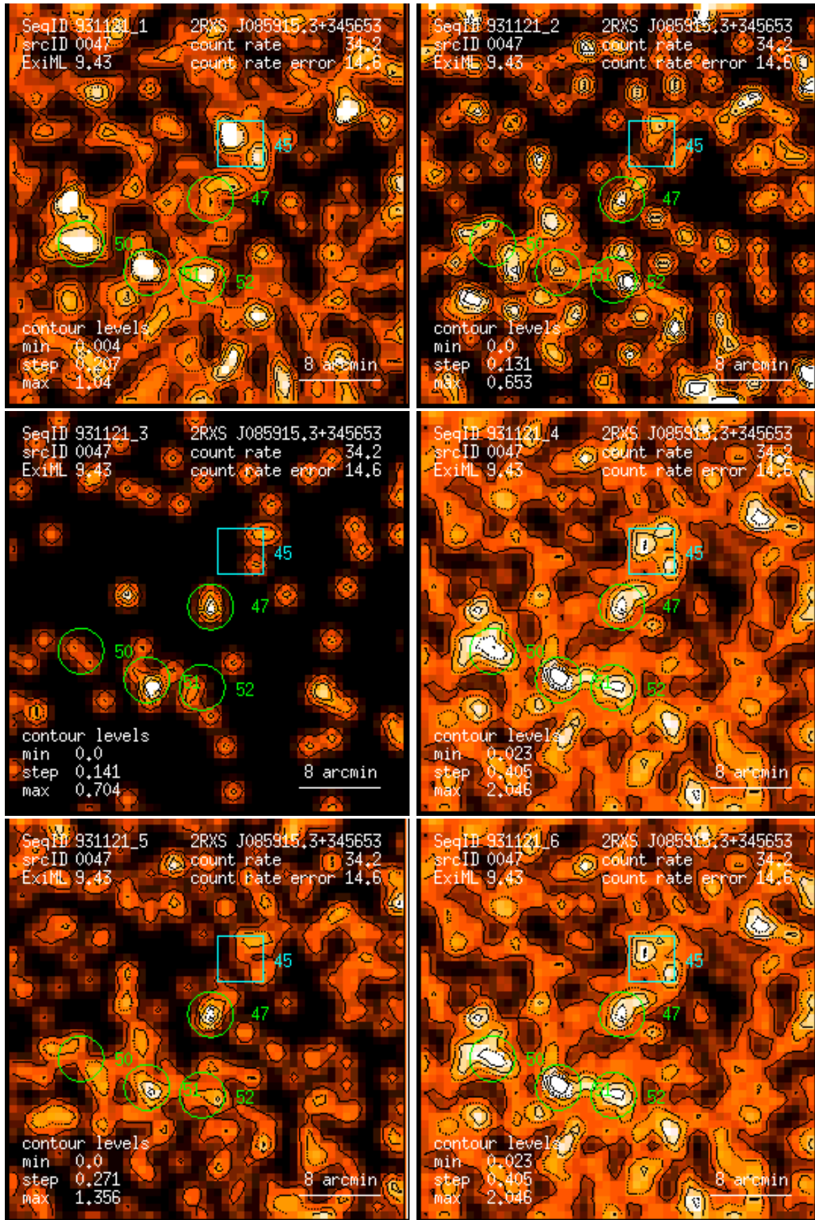
Figure 47: RASS 931121: detection 0047: band rate images, Gaussian filter: (1) PSPC channels 11 – 41, (2) 52 – 90, (3) 91 – 201, (4) 11 – 235, (5) 52 – 201, (6) 11 – 201. Broad band rates in counts/ks. Band rate contour levels in counts/ks/arcmin 2 .
