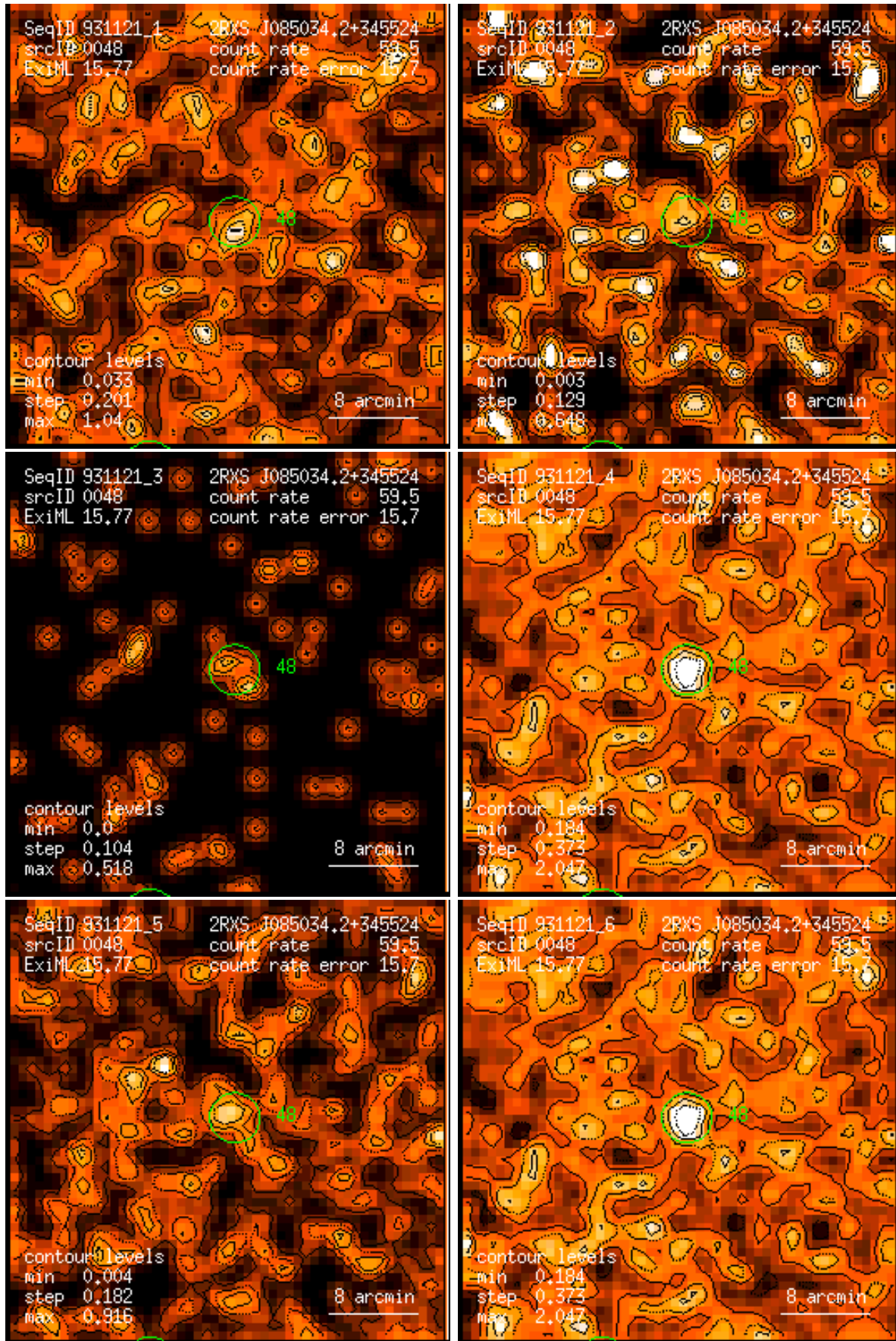
Figure 48: RASS 931121: detection 0048: band rate images, Gaussian filter: (1) PSPC channels 11 – 41, (2) 52 – 90, (3) 91 – 201, (4) 11 – 235, (5) 52 – 201, (6) 11 – 201. Broad band rates in counts/ks. Band rate contour levels in counts/ks/arcmin 2 .
