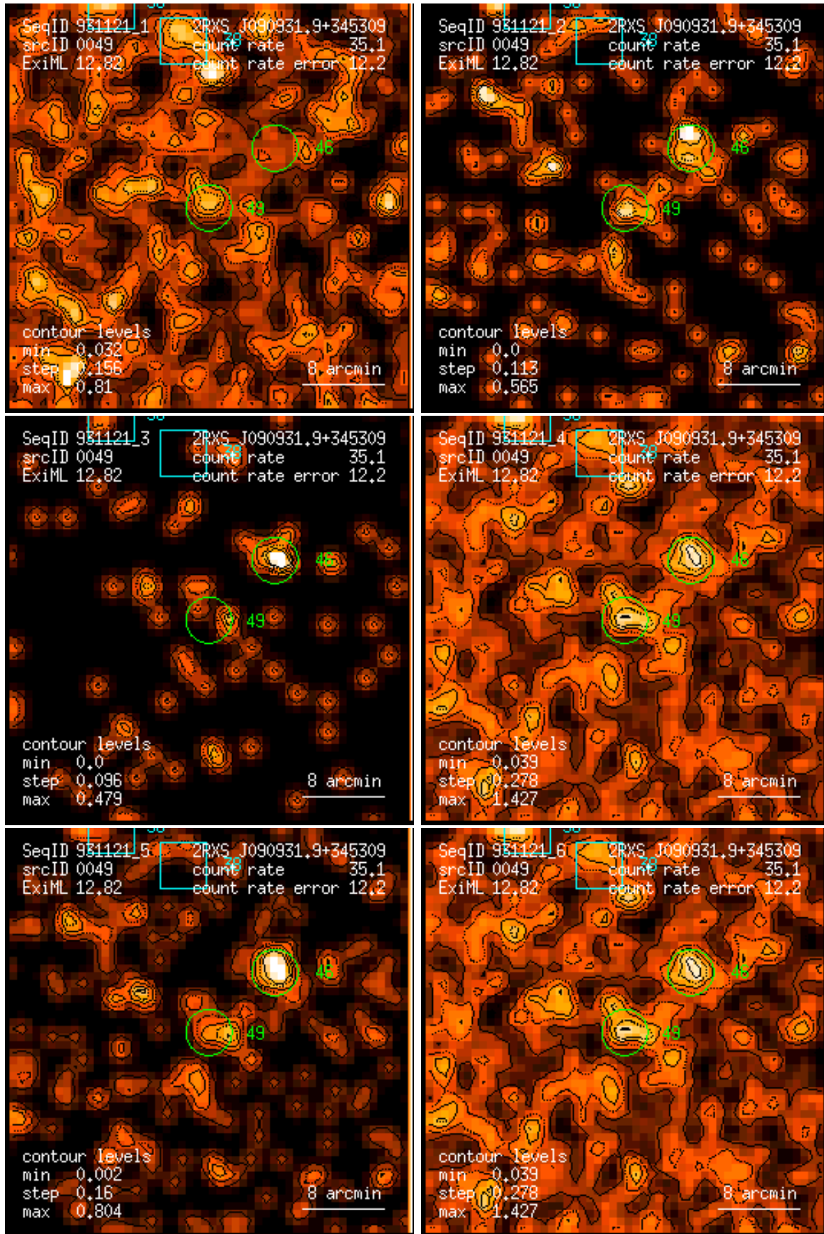
Figure 49: RASS 931121: detection 0049: band rate images, Gaussian filter: (1) PSPC channels 11 – 41, (2) 52 – 90, (3) 91 – 201, (4) 11 – 235, (5) 52 – 201, (6) 11 – 201. Broad band rates in counts/ks. Band rate contour levels in counts/ks/arcmin 2 .
