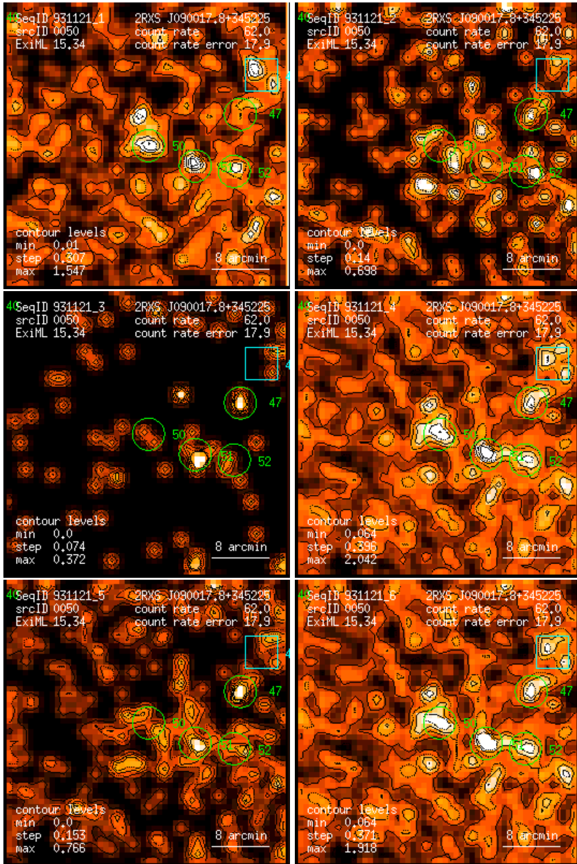
Figure 50: RASS 931121: detection 0050: band rate images, Gaussian filter: (1) PSPC channels 11 – 41, (2) 52 – 90, (3) 91 – 201, (4) 11 – 235, (5) 52 – 201, (6) 11 – 201. Broad band rates in counts/ks. Band rate contour levels in counts/ks/arcmin 2 .
