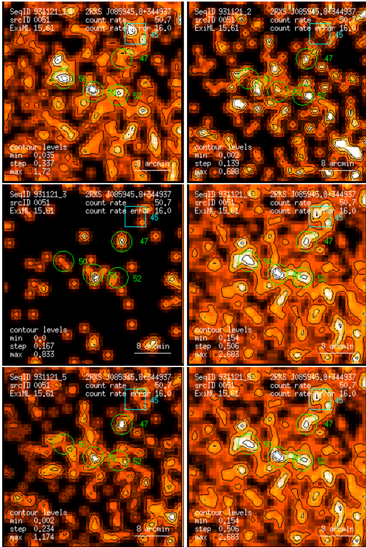
Figure 51: RASS 931121: detection 0051: band rate images, Gaussian filter: (1) PSPC channels 11 – 41, (2) 52 – 90, (3) 91 – 201, (4) 11 – 235, (5) 52 – 201, (6) 11 – 201. Broad band rates in counts/ks. Band rate contour levels in counts/ks/arcmin 2 .
