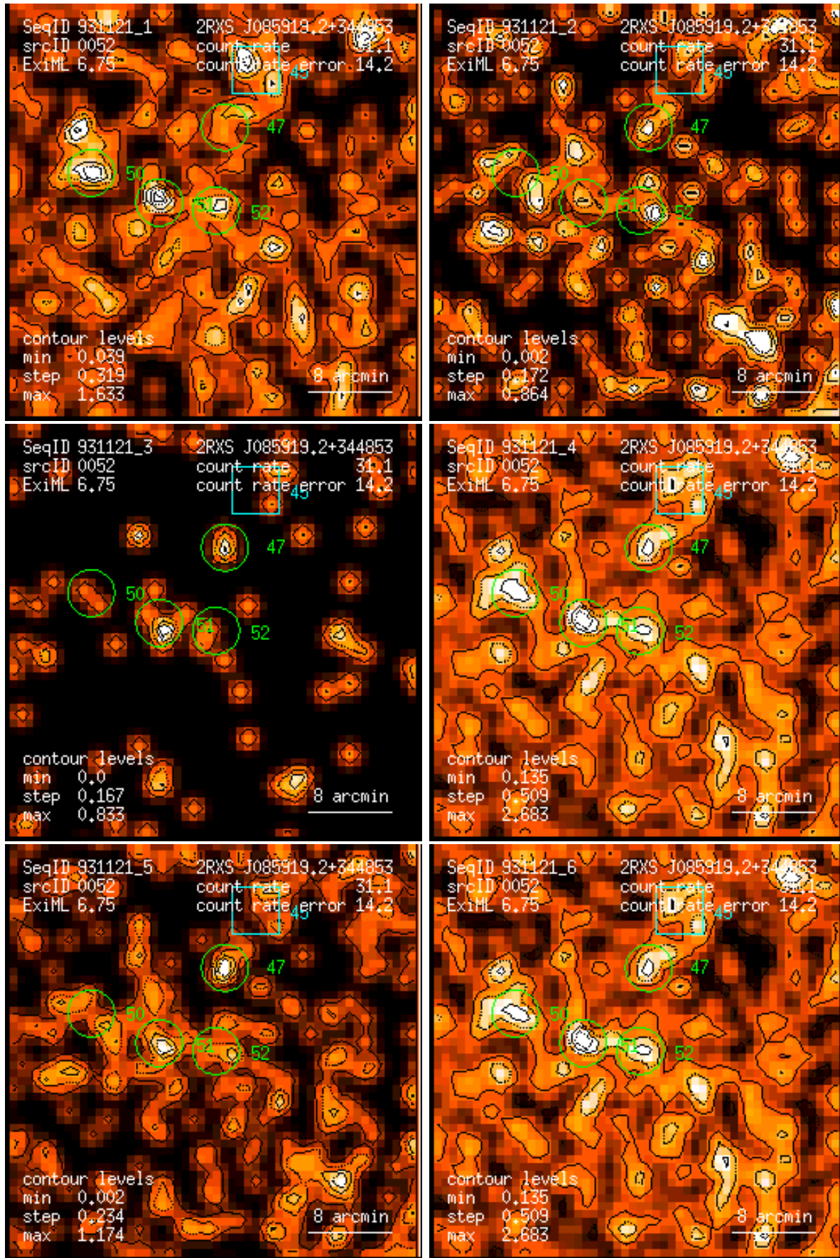
Figure 52: RASS 931121: detection 0052: band rate images, Gaussian filter: (1) PSPC channels 11 – 41, (2) 52 – 90, (3) 91 – 201, (4) 11 – 235, (5) 52 – 201, (6) 11 – 201. Broad band rates in counts/ks. Band rate contour levels in counts/ks/arcmin 2 .
