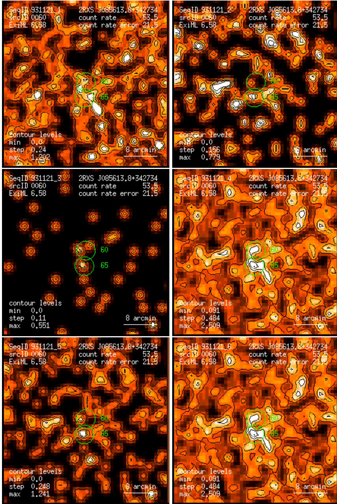
Figure 60: RASS 931121: detection 0060: band rate images, Gaussian filter: (1) PSPC channels 11 – 41, (2) 52 – 90, (3) 91 – 201, (4) 11 – 235, (5) 52 – 201, (6) 11 – 201. Broad band rates in counts/ks. Band rate contour levels in counts/ks/arcmin 2 .
