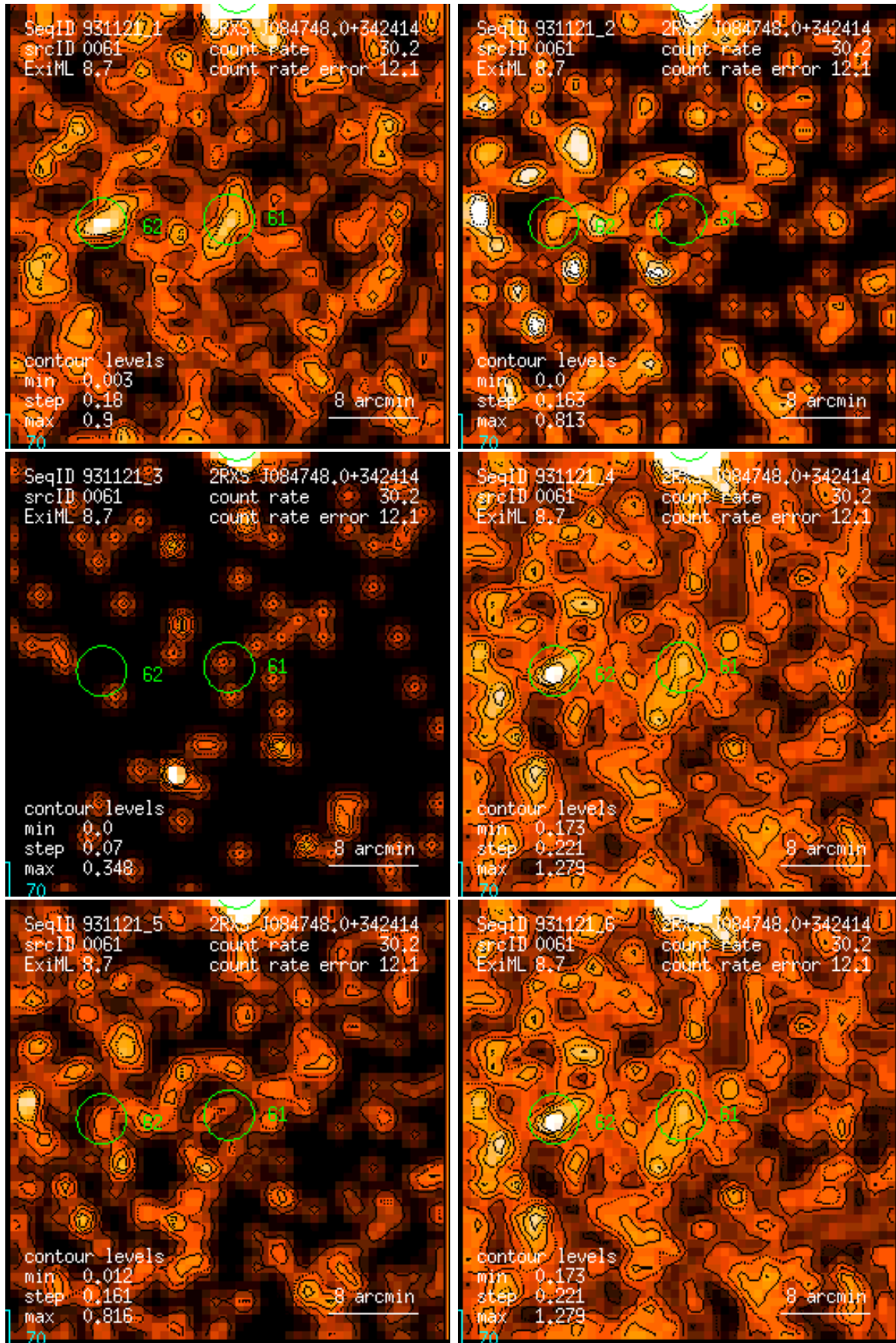
Figure 61: RASS 931121: detection 0061: band rate images, Gaussian filter: (1) PSPC channels 11 – 41, (2) 52 – 90, (3) 91 – 201, (4) 11 – 235, (5) 52 – 201, (6) 11 – 201. Broad band rates in counts/ks. Band rate contour levels in counts/ks/arcmin 2 .
