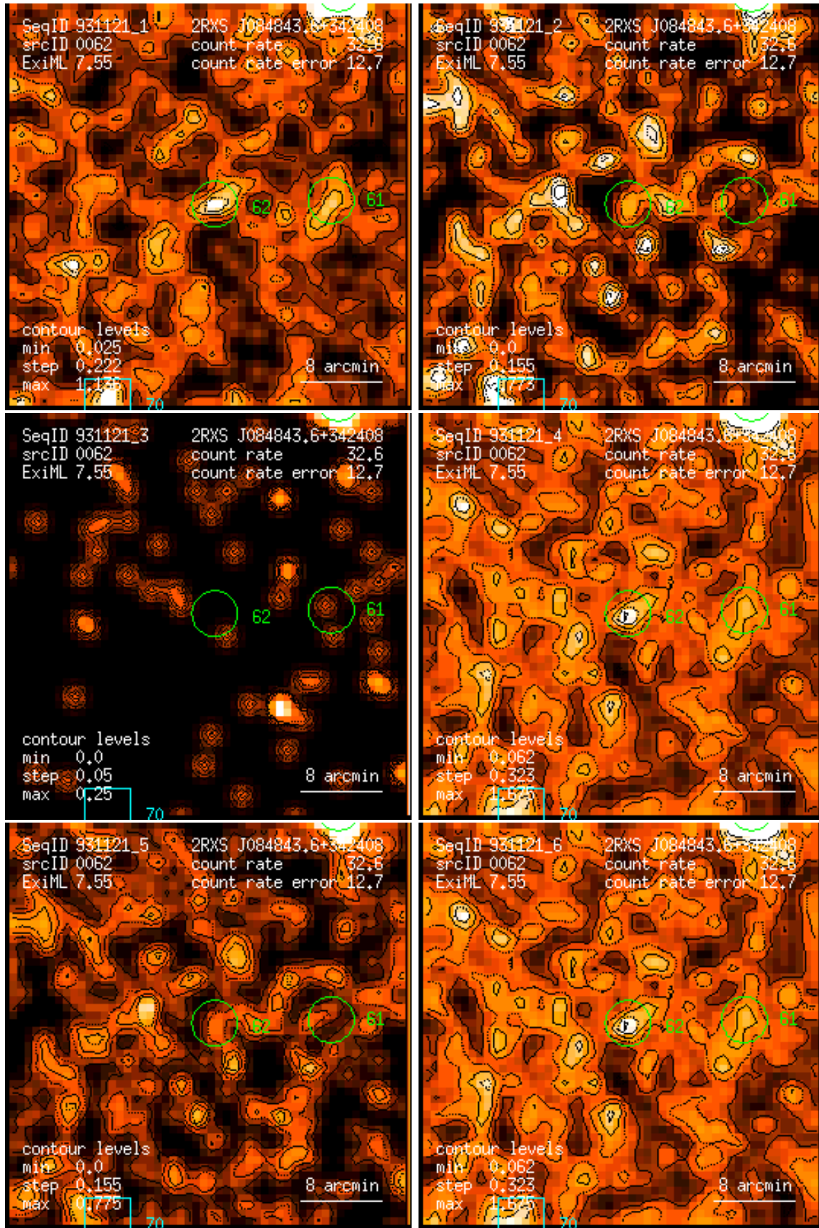
Figure 62: RASS 931121: detection 0062: band rate images, Gaussian filter: (1) PSPC channels 11 – 41, (2) 52 – 90, (3) 91 – 201, (4) 11 – 235, (5) 52 – 201, (6) 11 – 201. Broad band rates in counts/ks. Band rate contour levels in counts/ks/arcmin 2 .
