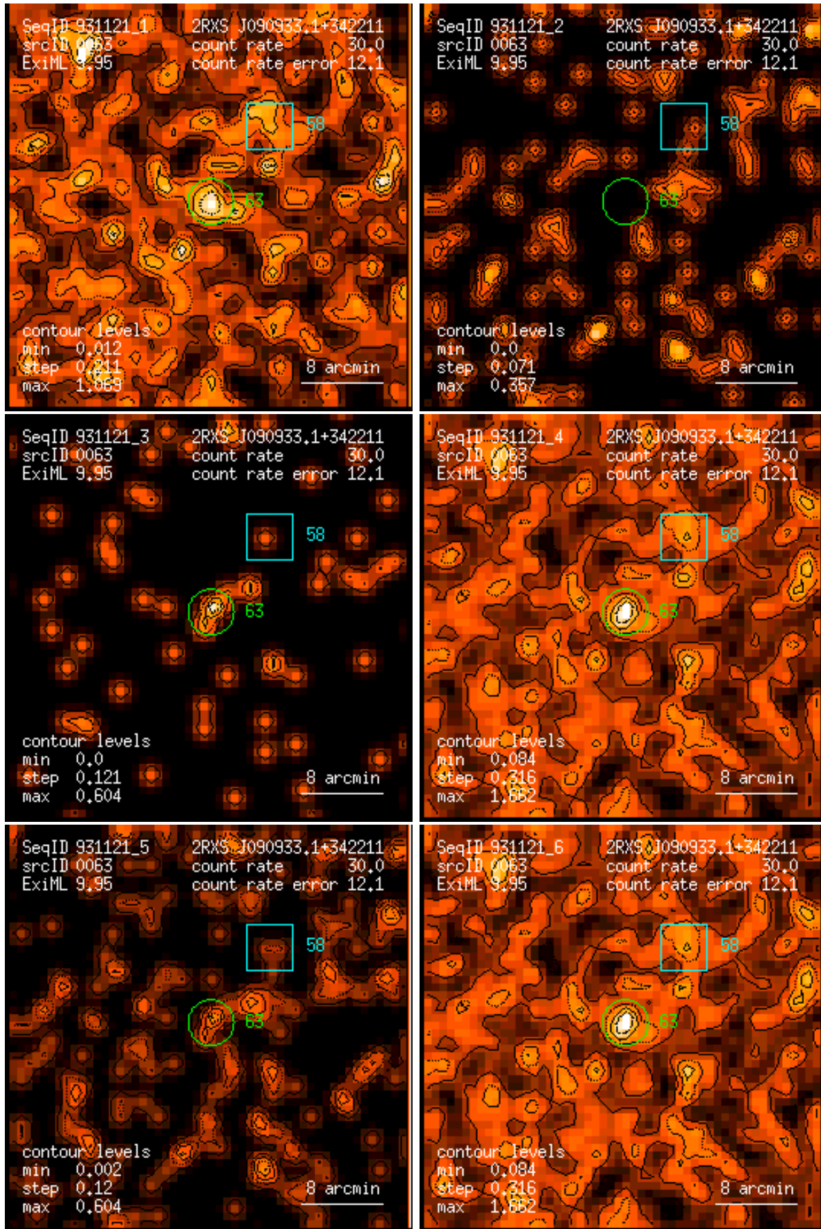
Figure 63: RASS 931121: detection 0063: band rate images, Gaussian filter: (1) PSPC channels 11 – 41, (2) 52 – 90, (3) 91 – 201, (4) 11 – 235, (5) 52 – 201, (6) 11 – 201. Broad band rates in counts/ks. Band rate contour levels in counts/ks/arcmin 2 .
