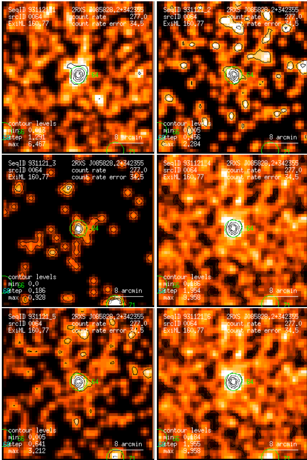
Figure 64: RASS 931121: detection 0064: band rate images, Gaussian filter: (1) PSPC channels 11 – 41, (2) 52 – 90, (3) 91 – 201, (4) 11 – 235, (5) 52 – 201, (6) 11 – 201. Broad band rates in counts/ks. Band rate contour levels in counts/ks/arcmin 2 .
