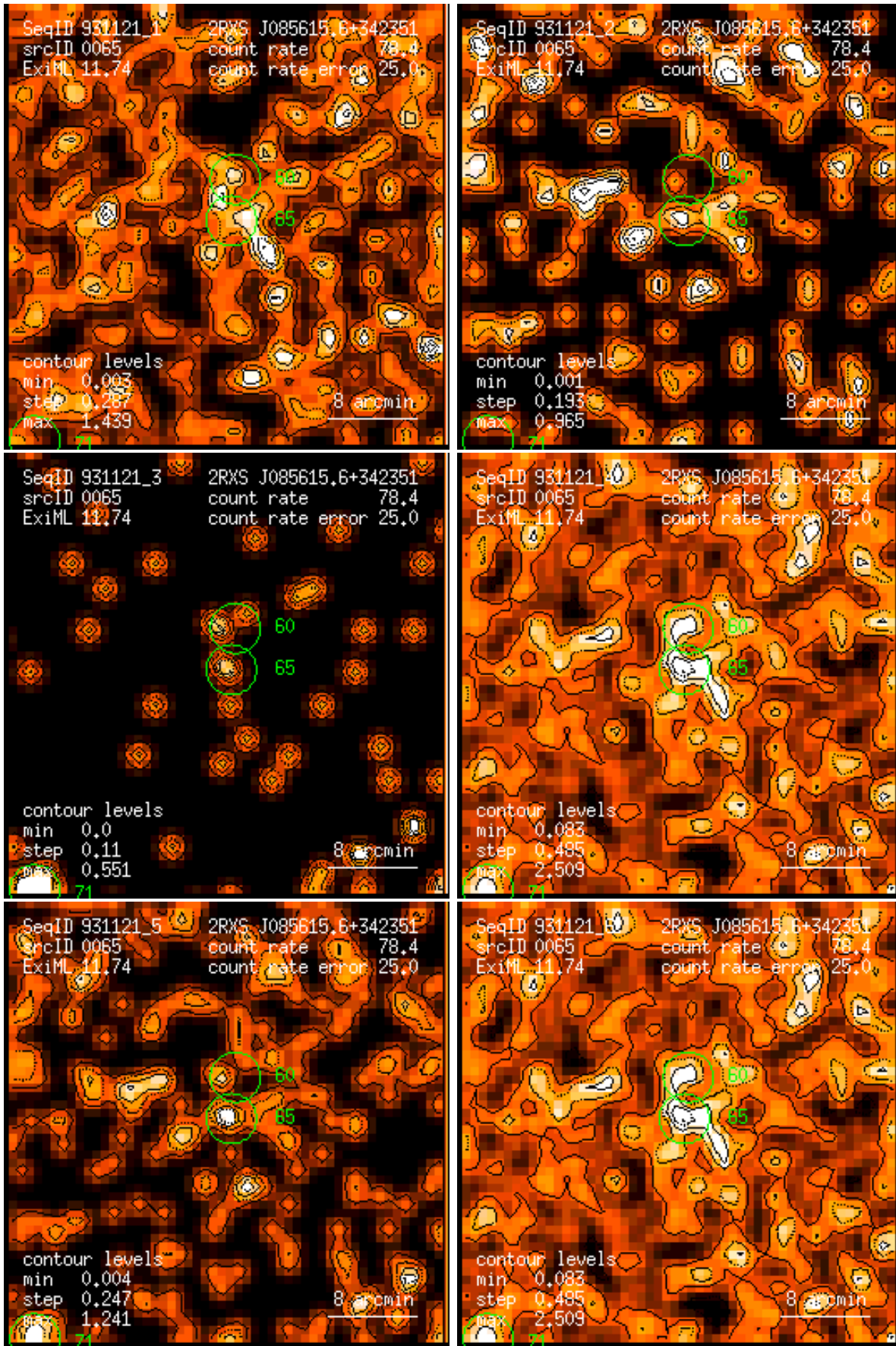
Figure 65: RASS 931121: detection 0065: band rate images, Gaussian filter: (1) PSPC channels 11 – 41, (2) 52 – 90, (3) 91 – 201, (4) 11 – 235, (5) 52 – 201, (6) 11 – 201. Broad band rates in counts/ks. Band rate contour levels in counts/ks/arcmin 2 .
