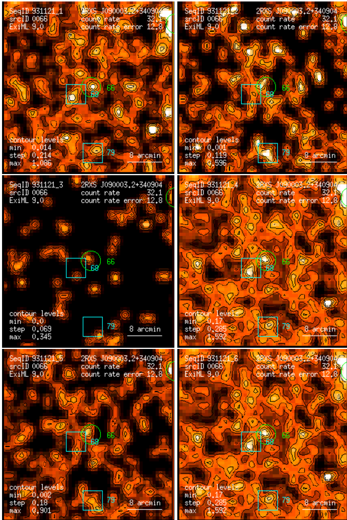
Figure 66: RASS 931121: detection 0066: band rate images, Gaussian filter: (1) PSPC channels 11 – 41, (2) 52 – 90, (3) 91 – 201, (4) 11 – 235, (5) 52 – 201, (6) 11 – 201. Broad band rates in counts/ks. Band rate contour levels in counts/ks/arcmin 2 .
