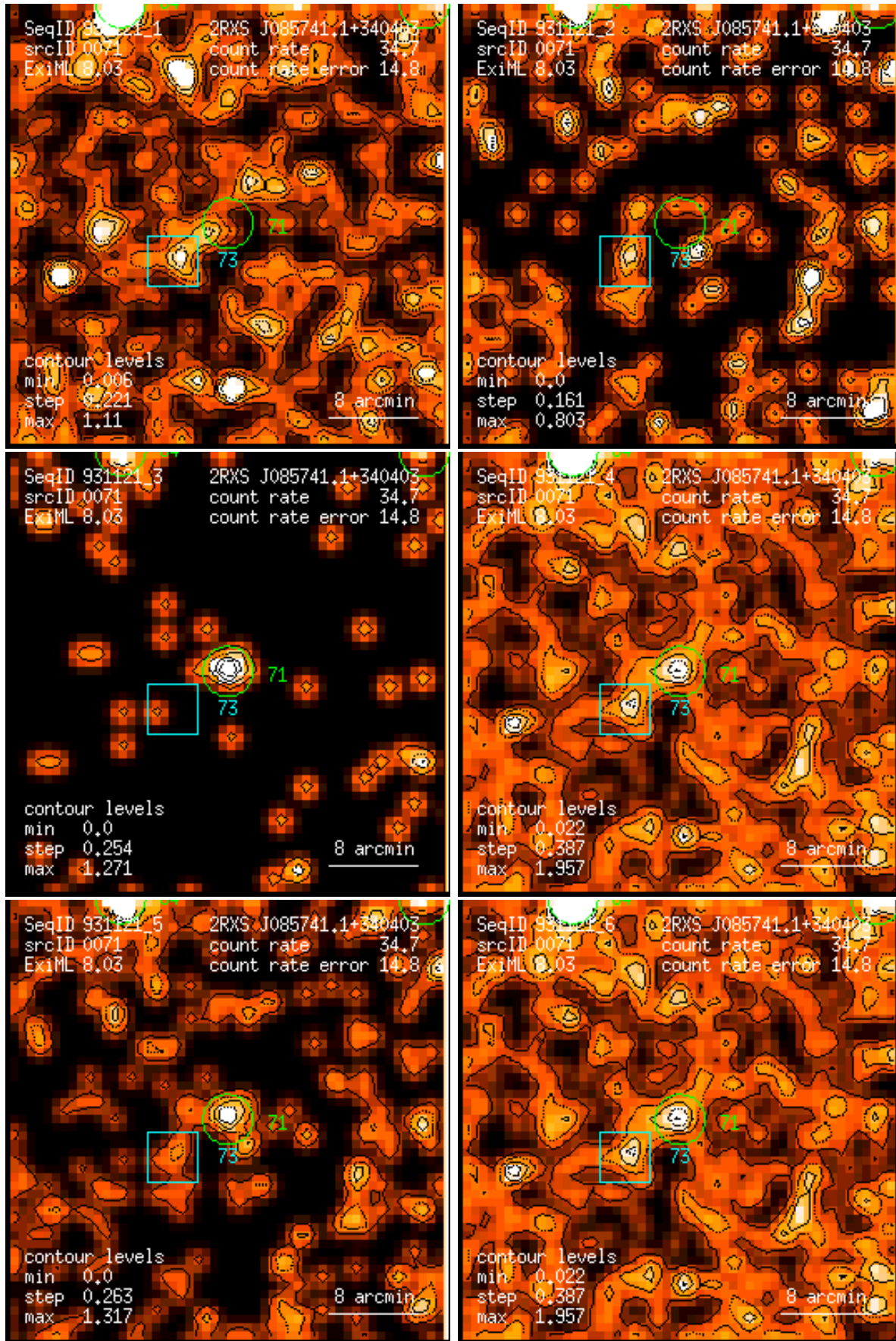
Figure 71: RASS 931121: detection 0071: band rate images, Gaussian filter: (1) PSPC channels 11 – 41, (2) 52 – 90, (3) 91 – 201, (4) 11 – 235, (5) 52 – 201, (6) 11 – 201. Broad band rates in counts/ks. Band rate contour levels in counts/ks/arcmin 2 .
