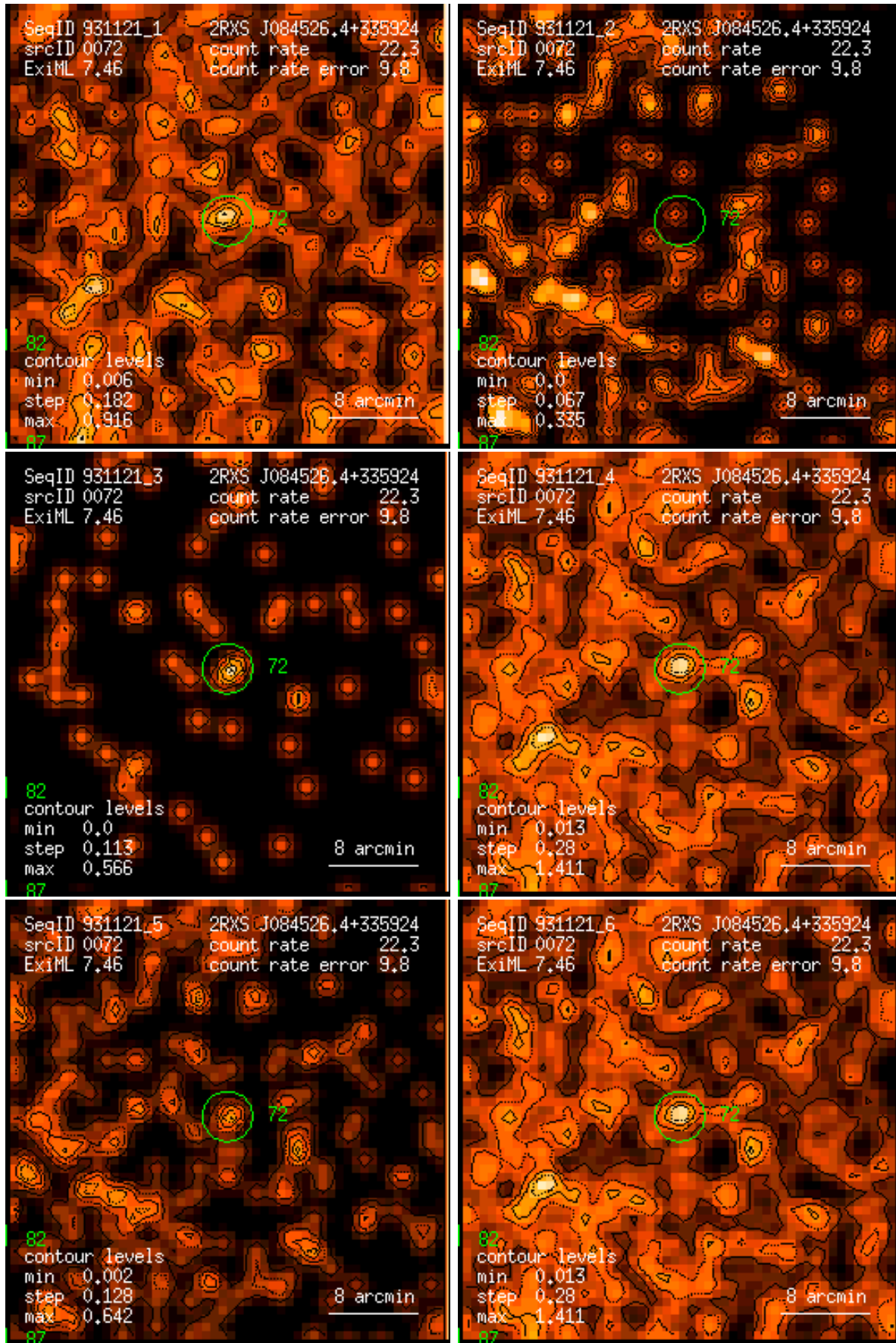
Figure 72: RASS 931121: detection 0072: band rate images, Gaussian filter: (1) PSPC channels 11 – 41, (2) 52 – 90, (3) 91 – 201, (4) 11 – 235, (5) 52 – 201, (6) 11 – 201. Broad band rates in counts/ks. Band rate contour levels in counts/ks/arcmin 2 .
