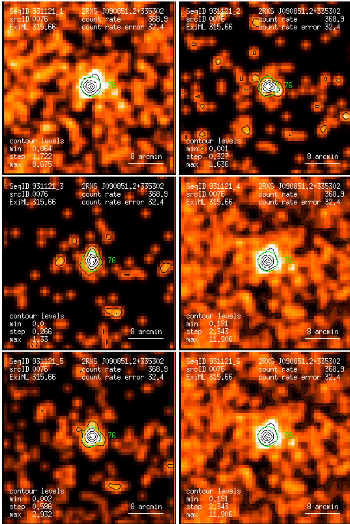
Figure 76: RASS 931121: detection 0076: band rate images, Gaussian filter: (1) PSPC channels 11 – 41, (2) 52 – 90, (3) 91 – 201, (4) 11 – 235, (5) 52 – 201, (6) 11 – 201. Broad band rates in counts/ks. Band rate contour levels in counts/ks/arcmin 2 .
