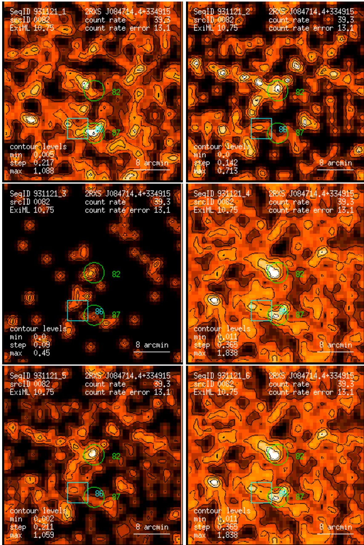
Figure 82: RASS 931121: detection 0082: band rate images, Gaussian filter: (1) PSPC channels 11 – 41, (2) 52 – 90, (3) 91 – 201, (4) 11 – 235, (5) 52 – 201, (6) 11 – 201. Broad band rates in counts/ks. Band rate contour levels in counts/ks/arcmin 2 .
