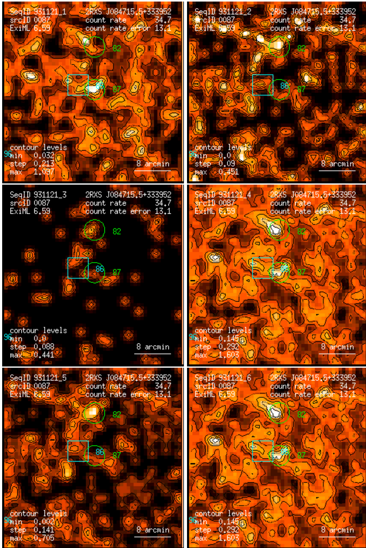
Figure 87: RASS 931121: detection 0087: band rate images, Gaussian filter: (1) PSPC channels 11 – 41, (2) 52 – 90, (3) 91 – 201, (4) 11 – 235, (5) 52 – 201, (6) 11 – 201. Broad band rates in counts/ks. Band rate contour levels in counts/ks/arcmin 2 .
