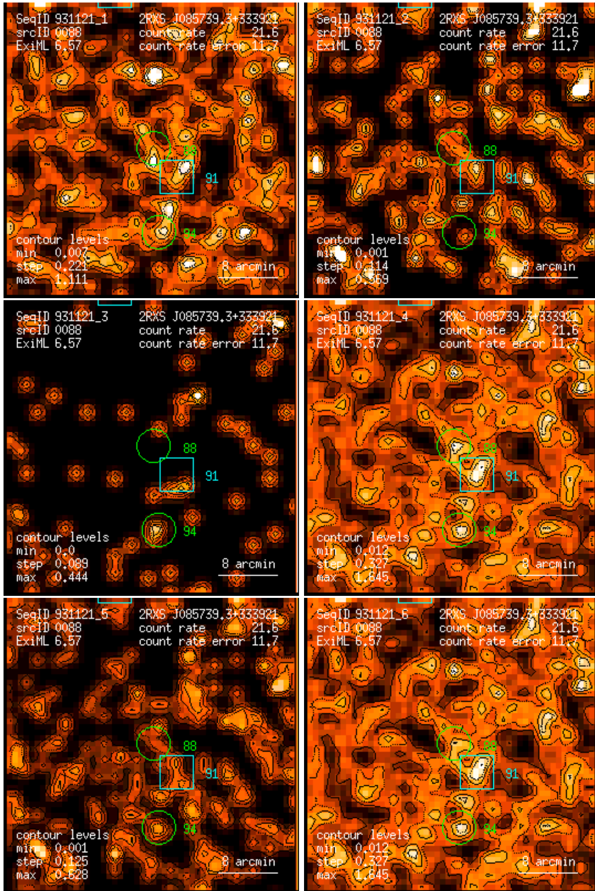
Figure 88: RASS 931121: detection 0088: band rate images, Gaussian filter: (1) PSPC channels 11 – 41, (2) 52 – 90, (3) 91 – 201, (4) 11 – 235, (5) 52 – 201, (6) 11 – 201. Broad band rates in counts/ks. Band rate contour levels in counts/ks/arcmin 2 .
