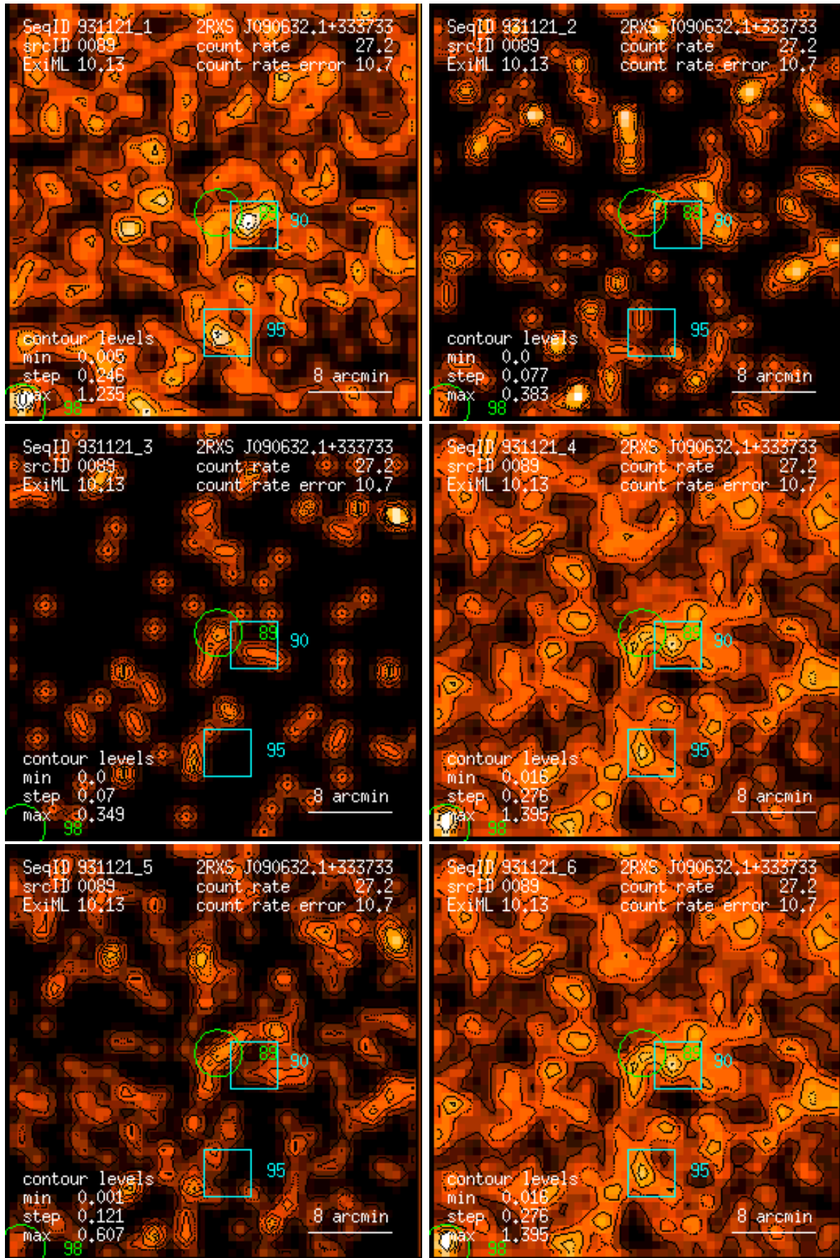
Figure 89: RASS 931121: detection 0089: band rate images, Gaussian filter: (1) PSPC channels 11 – 41, (2) 52 – 90, (3) 91 – 201, (4) 11 – 235, (5) 52 – 201, (6) 11 – 201. Broad band rates in counts/ks. Band rate contour levels in counts/ks/arcmin 2 .
