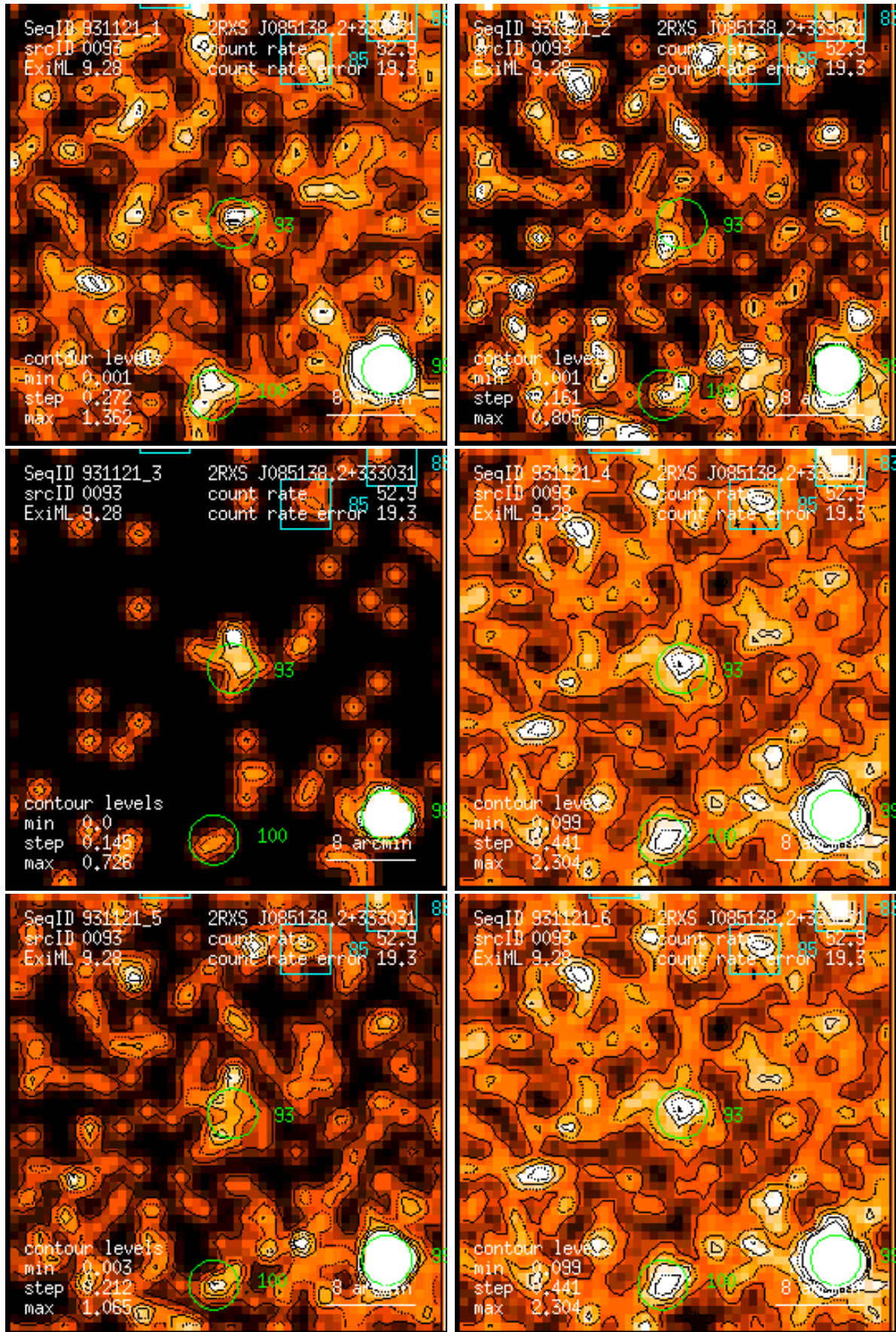
Figure 93: RASS 931121: detection 0093: band rate images, Gaussian filter: (1) PSPC channels 11 – 41, (2) 52 – 90, (3) 91 – 201, (4) 11 – 235, (5) 52 – 201, (6) 11 – 201. Broad band rates in counts/ks. Band rate contour levels in counts/ks/arcmin 2 .
