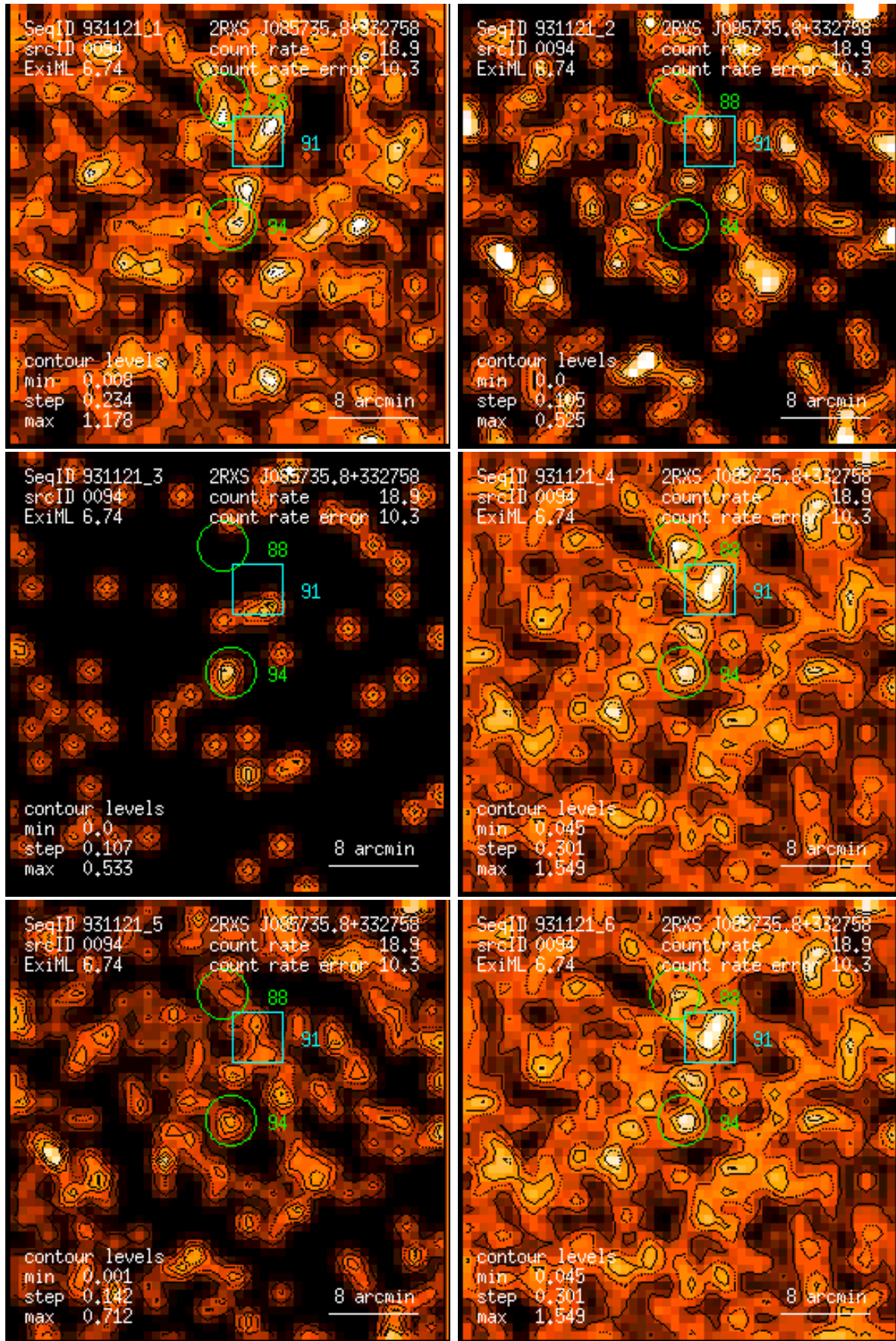
Figure 94: RASS 931121: detection 0094: band rate images, Gaussian filter: (1) PSPC channels 11 – 41, (2) 52 – 90, (3) 91 – 201, (4) 11 – 235, (5) 52 – 201, (6) 11 – 201. Broad band rates in counts/ks. Band rate contour levels in counts/ks/arcmin 2 .
