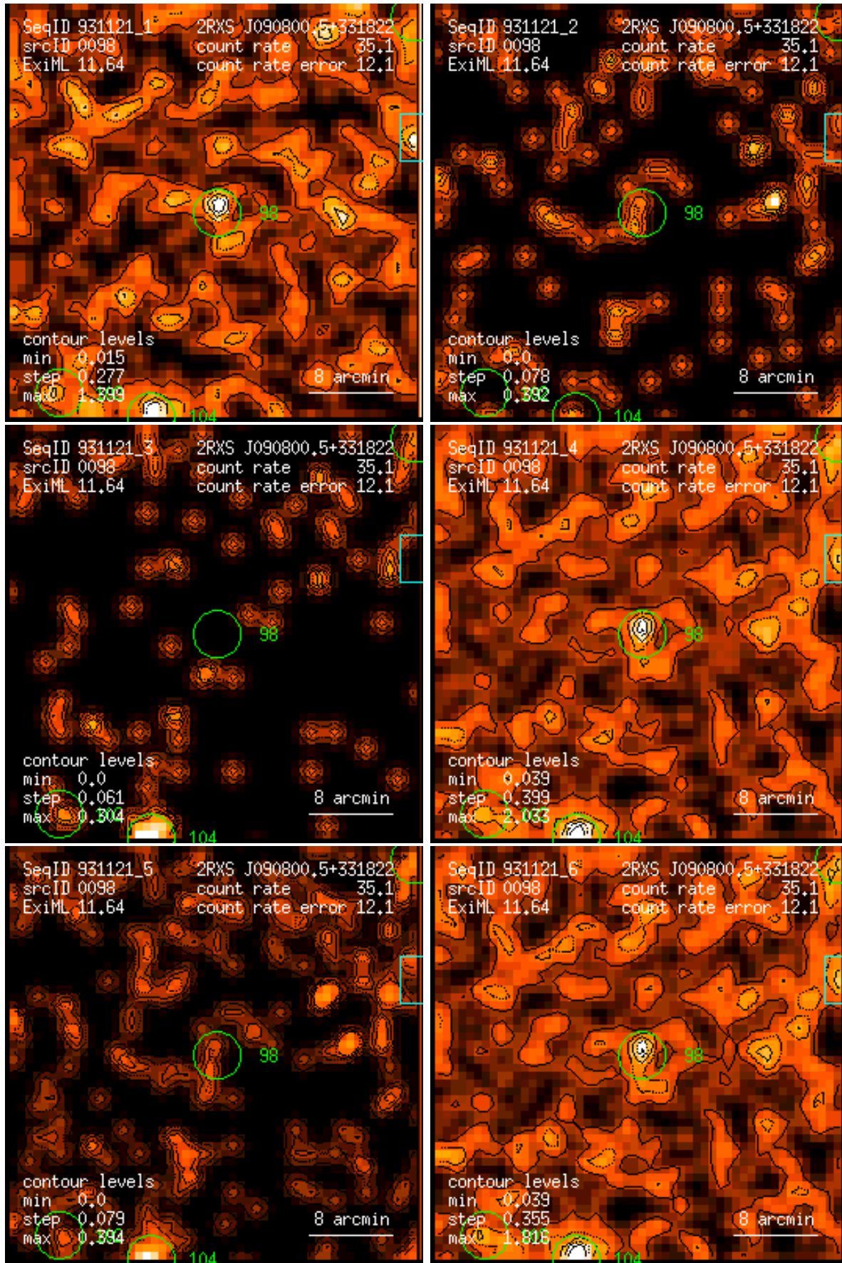
Figure 98: RASS 931121: detection 0098: band rate images, Gaussian filter: (1) PSPC channels 11 – 41, (2) 52 – 90, (3) 91 – 201, (4) 11 – 235, (5) 52 – 201, (6) 11 – 201. Broad band rates in counts/ks. Band rate contour levels in counts/ks/arcmin 2 .
