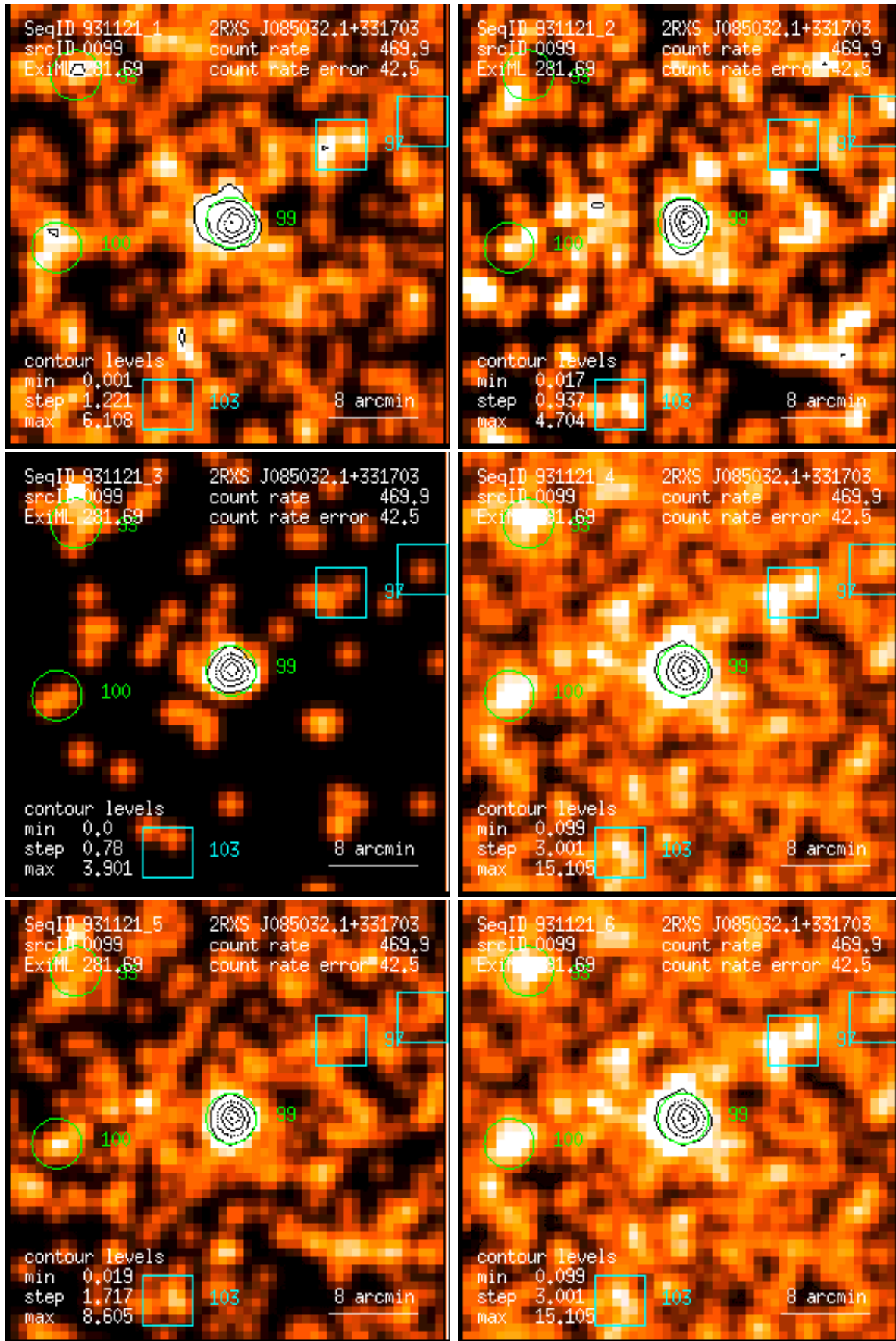
Figure 99: RASS 931121: detection 0099: band rate images, Gaussian filter: (1) PSPC channels 11 – 41, (2) 52 – 90, (3) 91 – 201, (4) 11 – 235, (5) 52 – 201, (6) 11 – 201. Broad band rates in counts/ks. Band rate contour levels in counts/ks/arcmin 2 .
