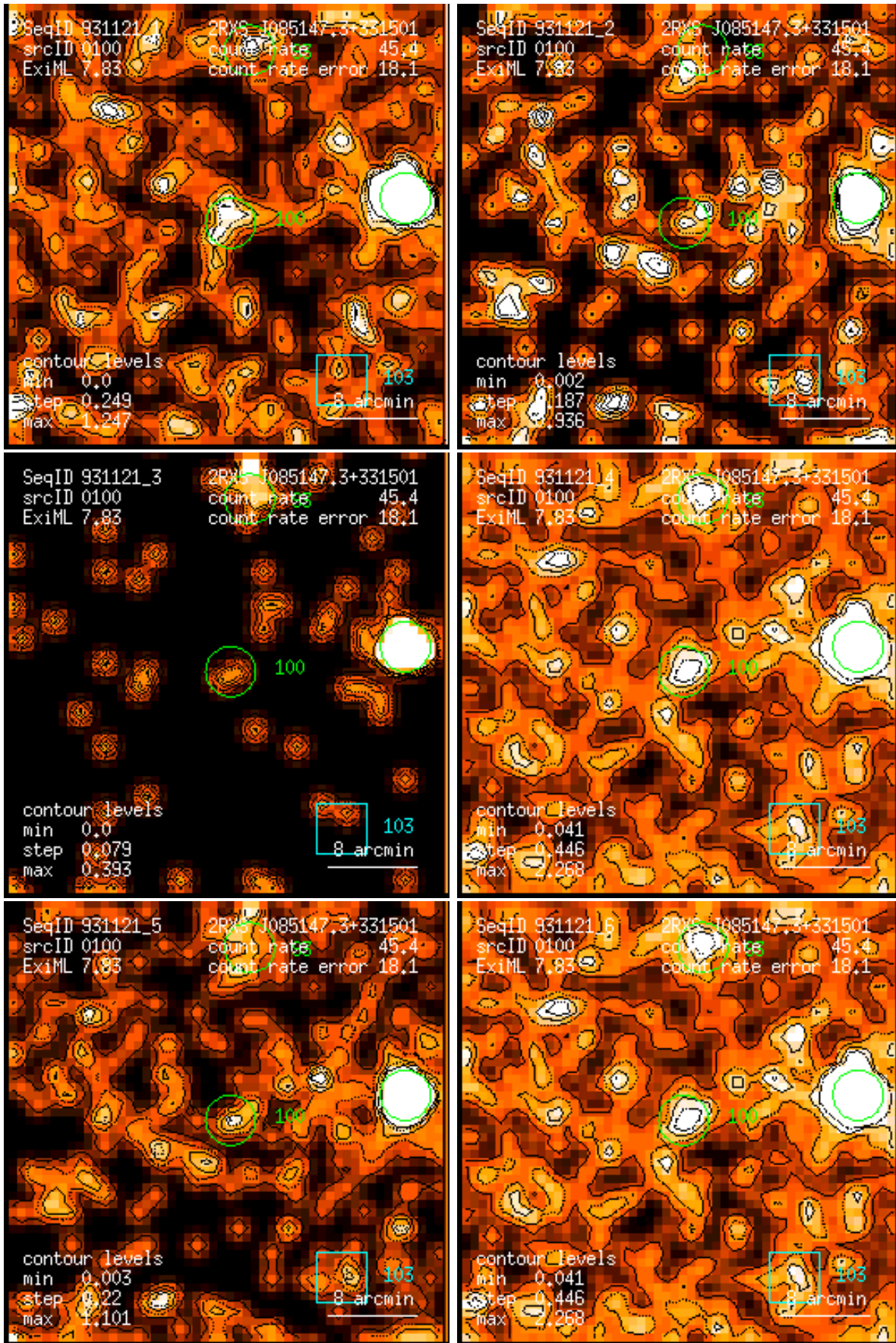
Figure 100: RASS 931121: detection 0100: band rate images, Gaussian filter: (1) PSPC channels 11 – 41, (2) 52 – 90, (3) 91 – 201, (4) 11 – 235, (5) 52 – 201, (6) 11 – 201. Broad band rates in counts/ks. Band rate contour levels in counts/ks/arcmin 2 .
