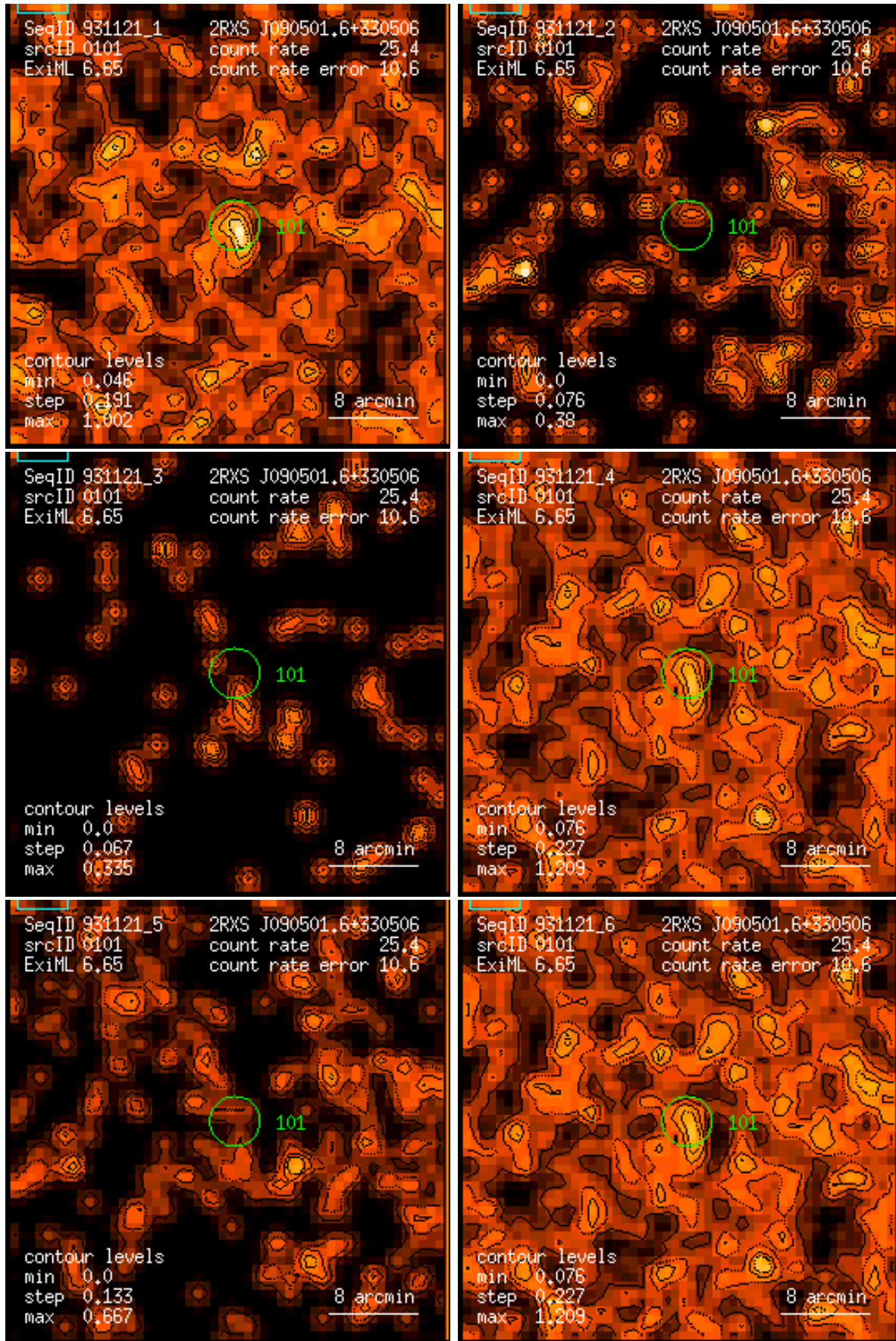
Figure 101: RASS 931121: detection 0101: band rate images, Gaussian filter: (1) PSPC channels 11 – 41, (2) 52 – 90, (3) 91 – 201, (4) 11 – 235, (5) 52 – 201, (6) 11 – 201. Broad band rates in counts/ks. Band rate contour levels in counts/ks/arcmin 2 .
