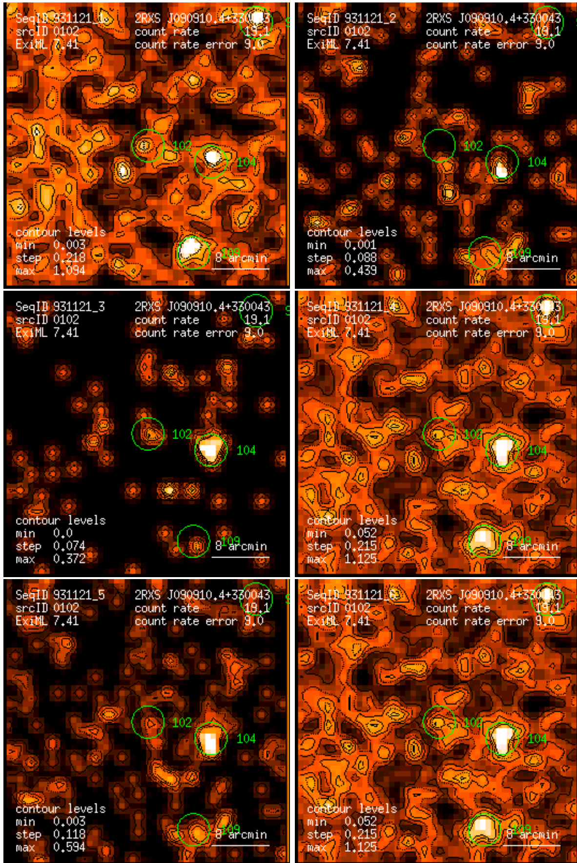
Figure 102: RASS 931121: detection 0102: band rate images, Gaussian filter: (1) PSPC channels 11 – 41, (2) 52 – 90, (3) 91 – 201, (4) 11 – 235, (5) 52 – 201, (6) 11 – 201. Broad band rates in counts/ks. Band rate contour levels in counts/ks/arcmin 2 .
