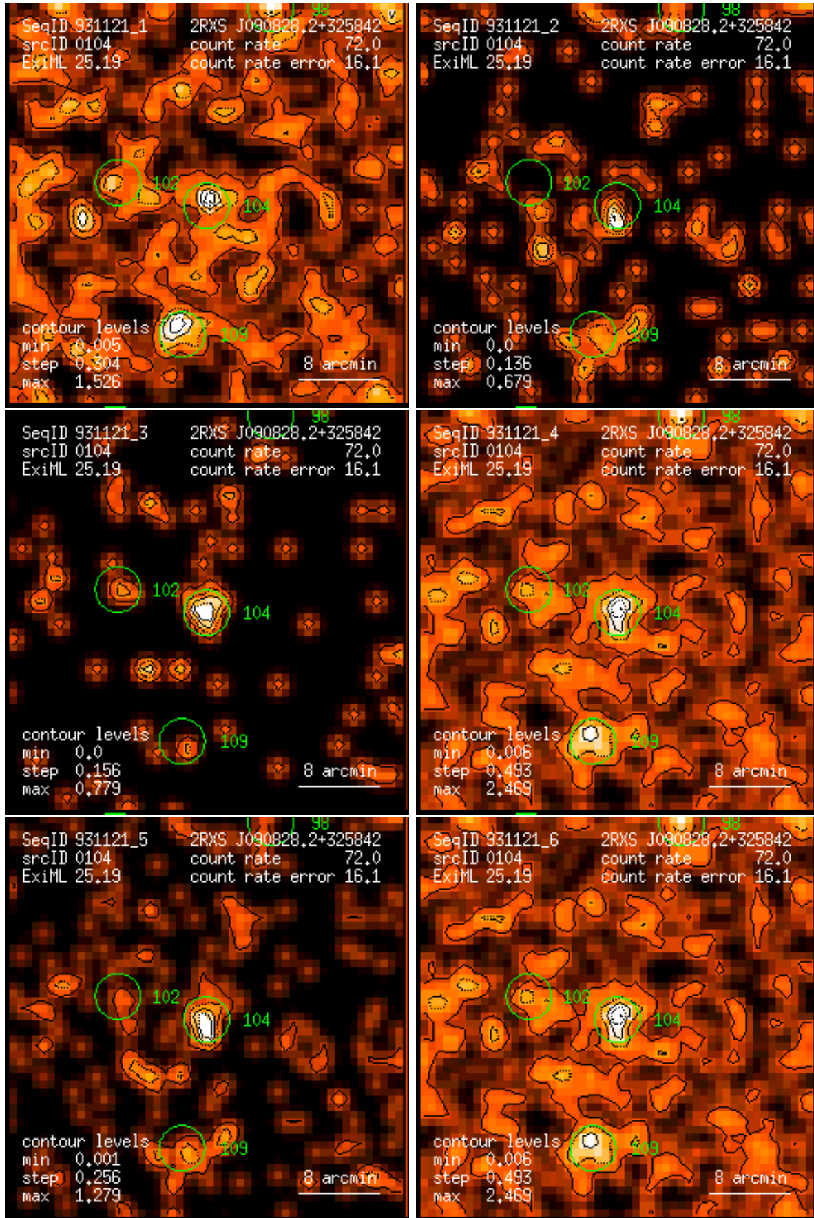
Figure 104: RASS 931121: detection 0104: band rate images, Gaussian filter: (1) PSPC channels 11 – 41, (2) 52 – 90, (3) 91 – 201, (4) 11 – 235, (5) 52 – 201, (6) 11 – 201. Broad band rates in counts/ks. Band rate contour levels in counts/ks/arcmin 2 .
