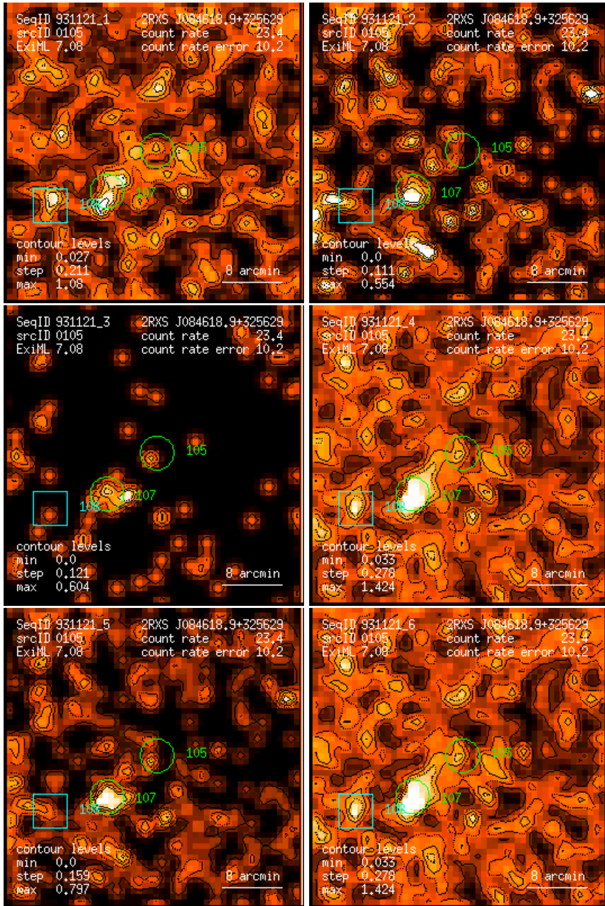
Figure 105: RASS 931121: detection 0105: band rate images, Gaussian filter: (1) PSPC channels 11 – 41, (2) 52 – 90, (3) 91 – 201, (4) 11 – 235, (5) 52 – 201, (6) 11 – 201. Broad band rates in counts/ks. Band rate contour levels in counts/ks/arcmin 2 .
