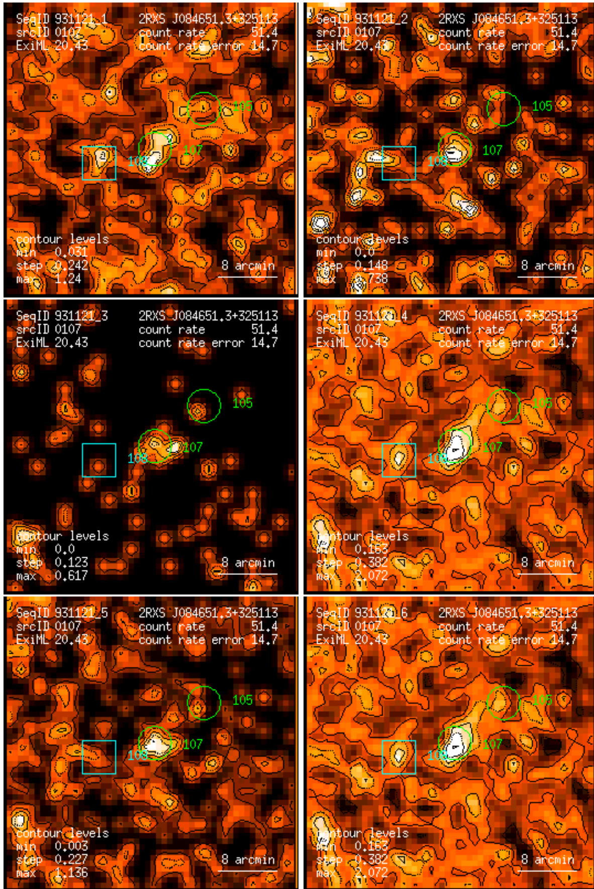
Figure 107: RASS 931121: detection 0107: band rate images, Gaussian filter: (1) PSPC channels 11 – 41, (2) 52 – 90, (3) 91 – 201, (4) 11 – 235, (5) 52 – 201, (6) 11 – 201. Broad band rates in counts/ks. Band rate contour levels in counts/ks/arcmin 2 .
