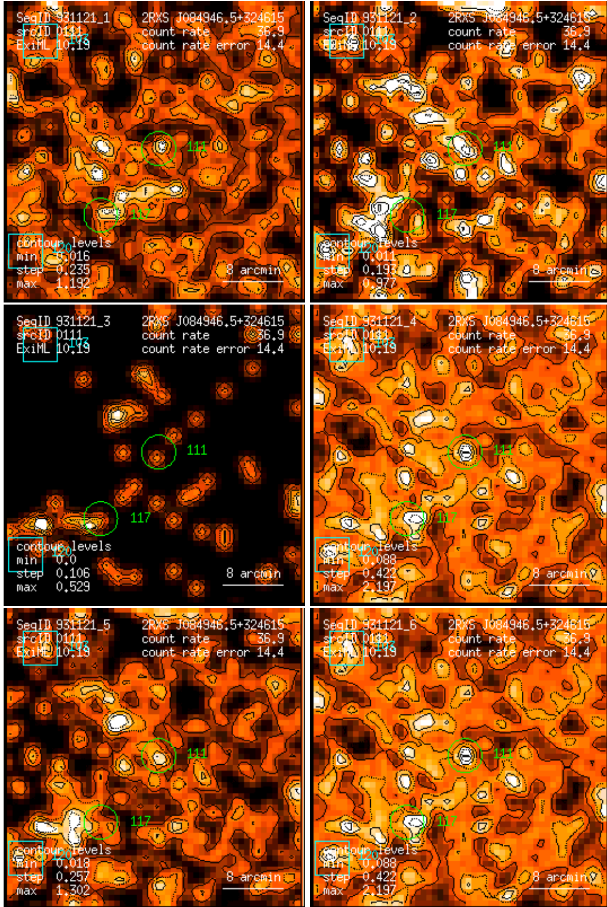
Figure 111: RASS 931121: detection 0111: band rate images, Gaussian filter: (1) PSPC channels 11 – 41, (2) 52 – 90, (3) 91 – 201, (4) 11 – 235, (5) 52 – 201, (6) 11 – 201. Broad band rates in counts/ks. Band rate contour levels in counts/ks/arcmin 2 .
