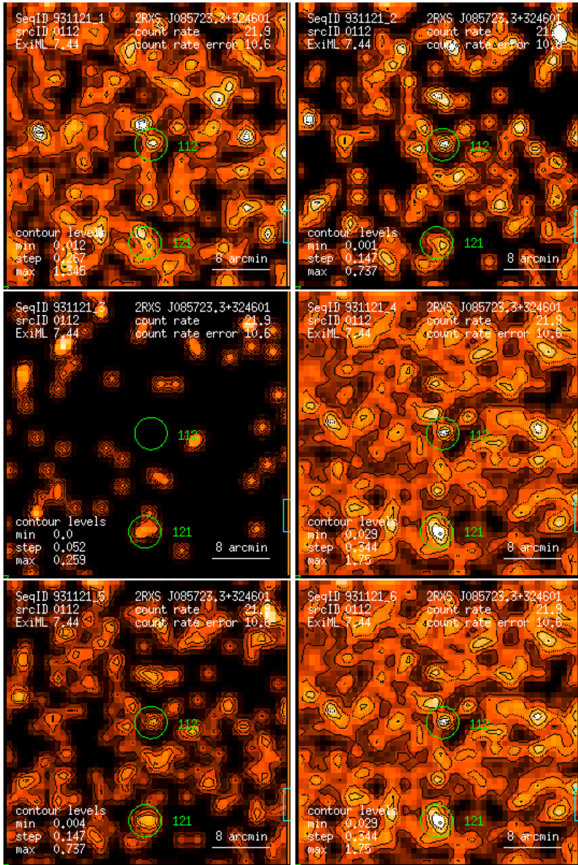
Figure 112: RASS 931121: detection 0112: band rate images, Gaussian filter: (1) PSPC channels 11 – 41, (2) 52 – 90, (3) 91 – 201, (4) 11 – 235, (5) 52 – 201, (6) 11 – 201. Broad band rates in counts/ks. Band rate contour levels in counts/ks/arcmin 2 .
