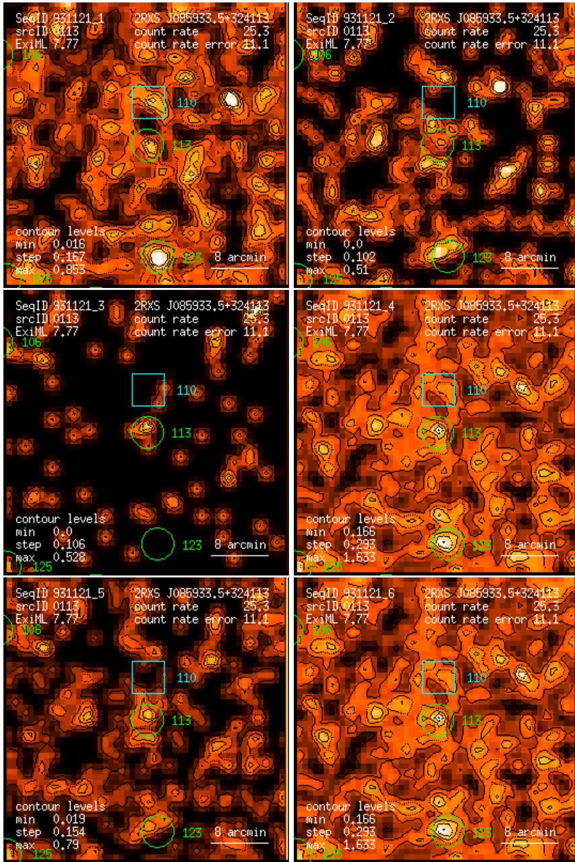
Figure 113: RASS 931121: detection 0113: band rate images, Gaussian filter: (1) PSPC channels 11 – 41, (2) 52 – 90, (3) 91 – 201, (4) 11 – 235, (5) 52 – 201, (6) 11 – 201. Broad band rates in counts/ks. Band rate contour levels in counts/ks/arcmin 2 .
