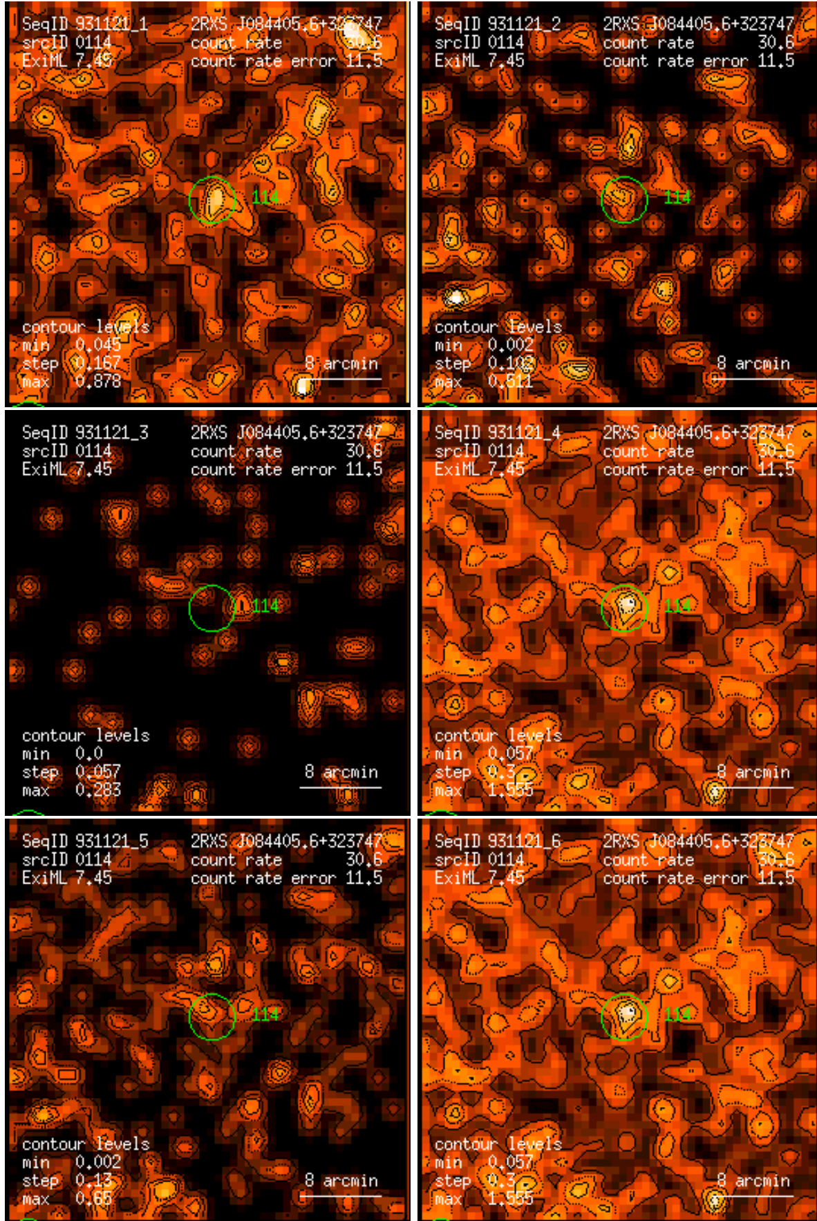
Figure 114: RASS 931121: detection 0114: band rate images, Gaussian filter: (1) PSPC channels 11 – 41, (2) 52 – 90, (3) 91 – 201, (4) 11 – 235, (5) 52 – 201, (6) 11 – 201. Broad band rates in counts/ks. Band rate contour levels in counts/ks/arcmin 2 .
