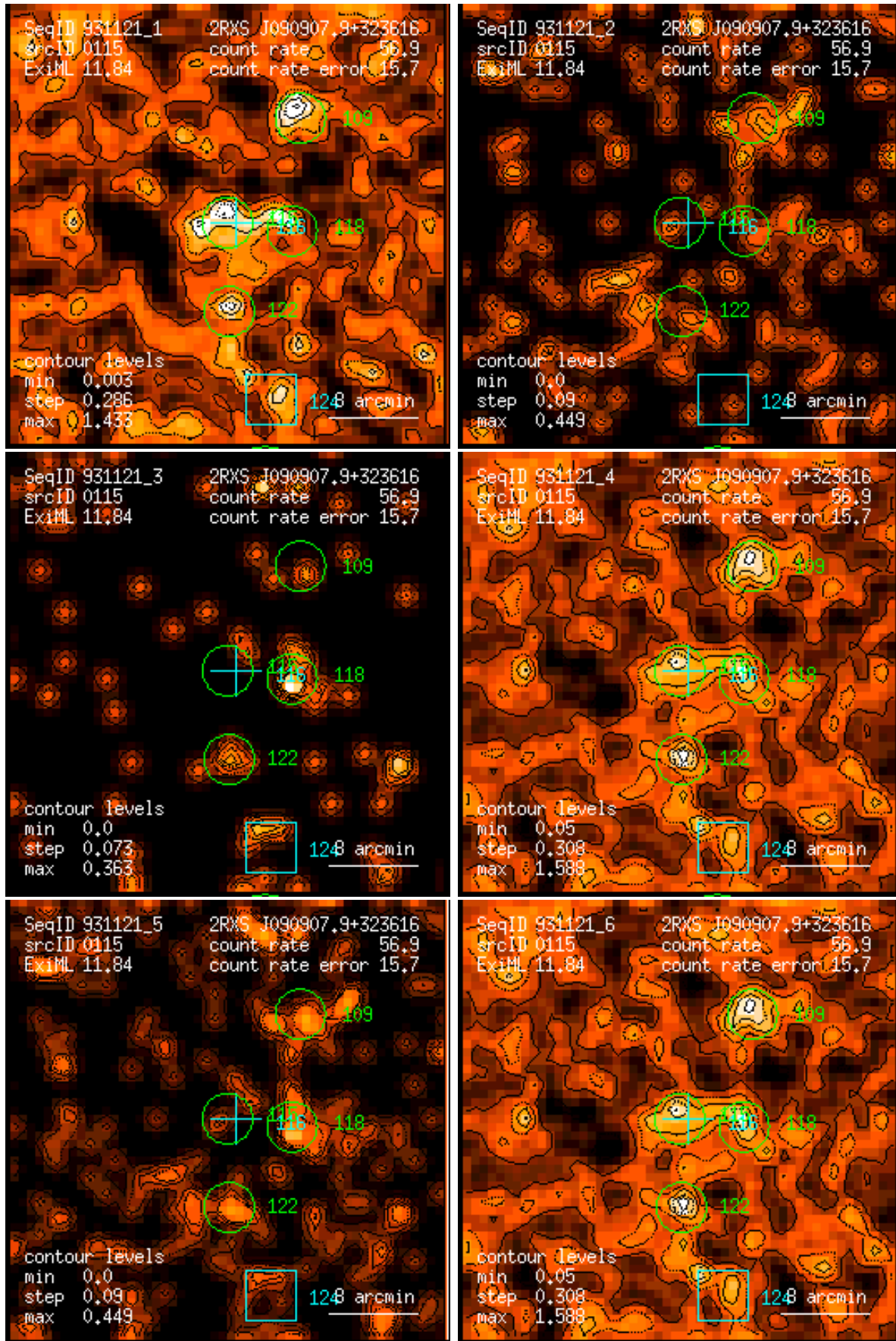
Figure 115: RASS 931121: detection 0115: band rate images, Gaussian filter: (1) PSPC channels 11 – 41, (2) 52 – 90, (3) 91 – 201, (4) 11 – 235, (5) 52 – 201, (6) 11 – 201. Broad band rates in counts/ks. Band rate contour levels in counts/ks/arcmin 2 .
