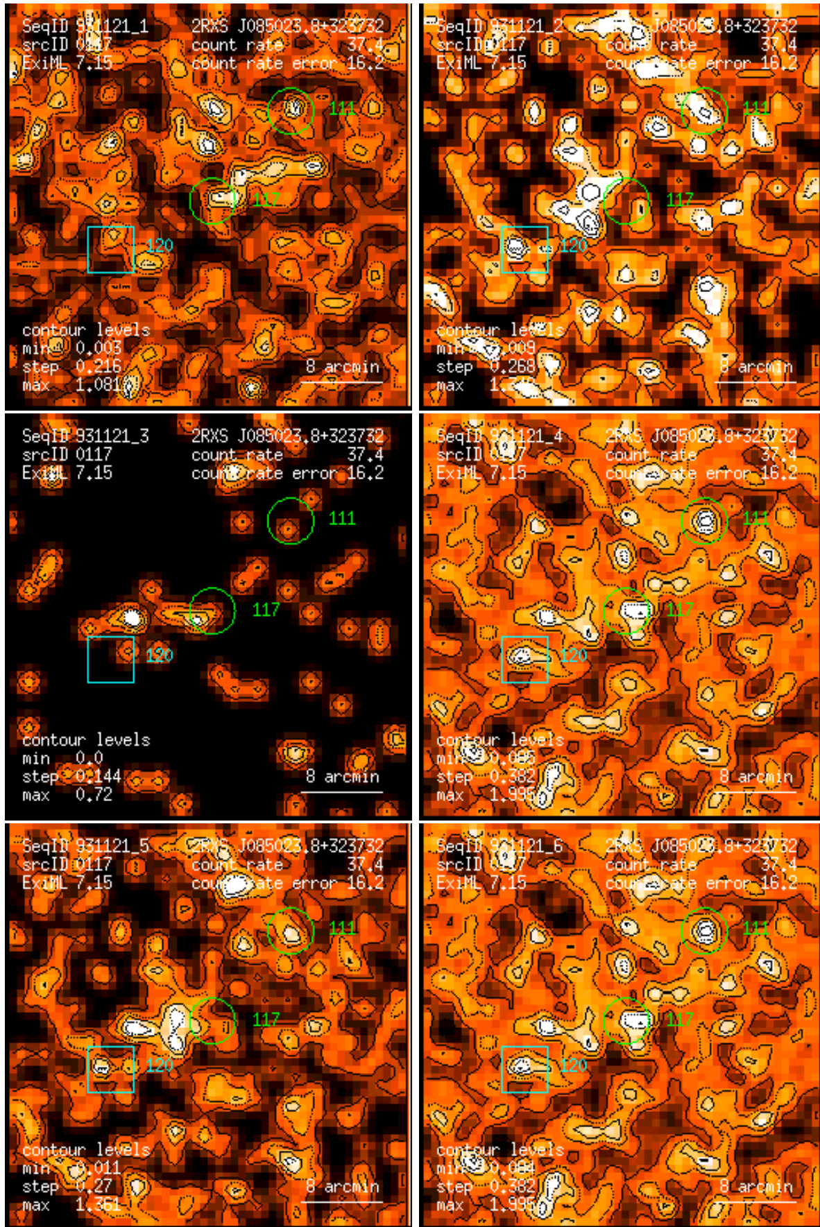
Figure 117: RASS 931121: detection 0117: band rate images, Gaussian filter: (1) PSPC channels 11 – 41, (2) 52 – 90, (3) 91 – 201, (4) 11 – 235, (5) 52 – 201, (6) 11 – 201. Broad band rates in counts/ks. Band rate contour levels in counts/ks/arcmin 2 .
