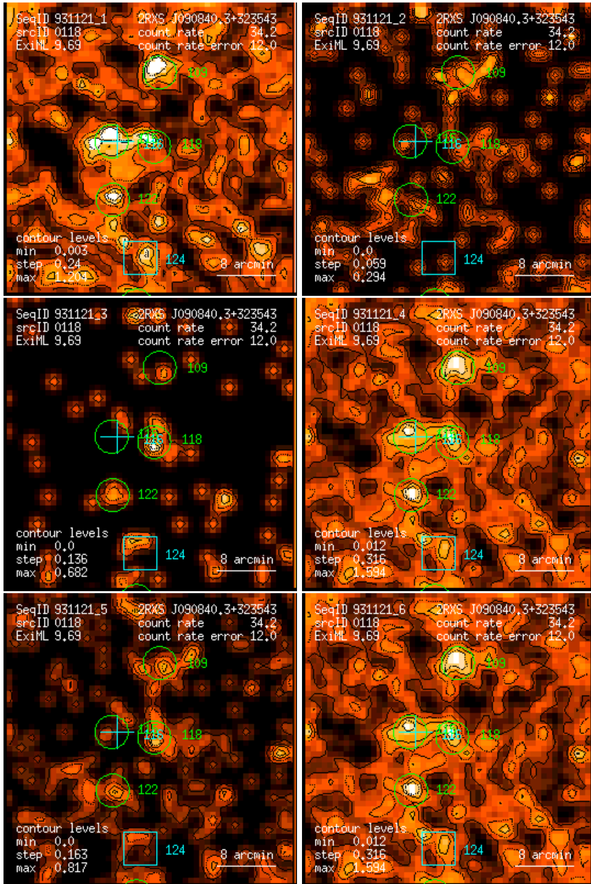
Figure 118: RASS 931121: detection 0118: band rate images, Gaussian filter: (1) PSPC channels 11 – 41, (2) 52 – 90, (3) 91 – 201, (4) 11 – 235, (5) 52 – 201, (6) 11 – 201. Broad band rates in counts/ks. Band rate contour levels in counts/ks/arcmin 2 .
