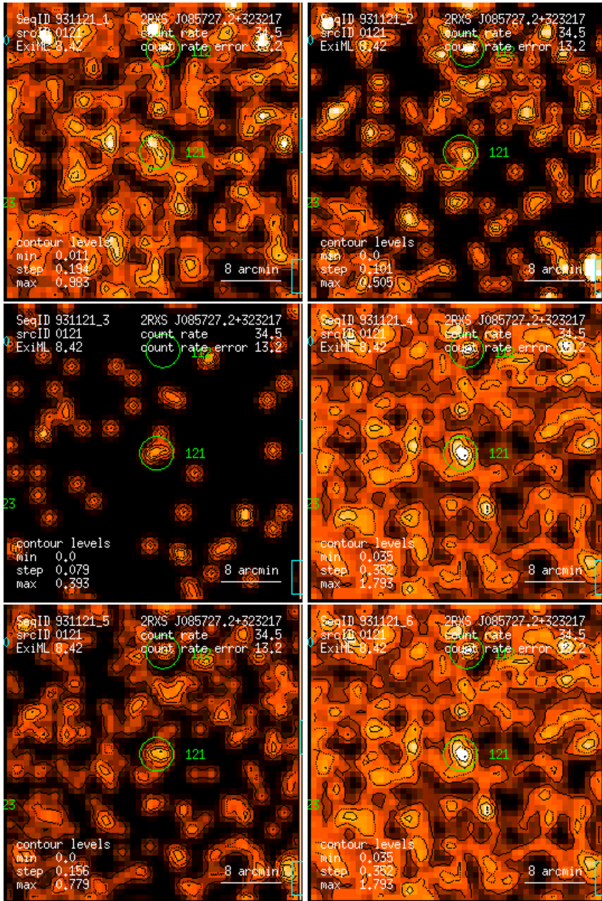
Figure 121: RASS 931121: detection 0121: band rate images, Gaussian filter: (1) PSPC channels 11 – 41, (2) 52 – 90, (3) 91 – 201, (4) 11 – 235, (5) 52 – 201, (6) 11 – 201. Broad band rates in counts/ks. Band rate contour levels in counts/ks/arcmin 2 .
