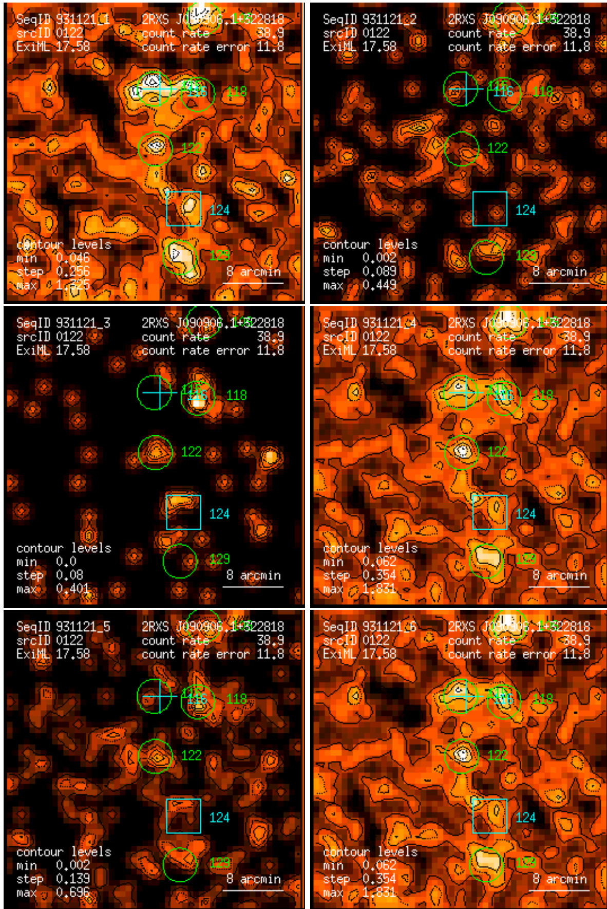
Figure 122: RASS 931121: detection 0122: band rate images, Gaussian filter: (1) PSPC channels 11 – 41, (2) 52 – 90, (3) 91 – 201, (4) 11 – 235, (5) 52 – 201, (6) 11 – 201. Broad band rates in counts/ks. Band rate contour levels in counts/ks/arcmin 2 .
