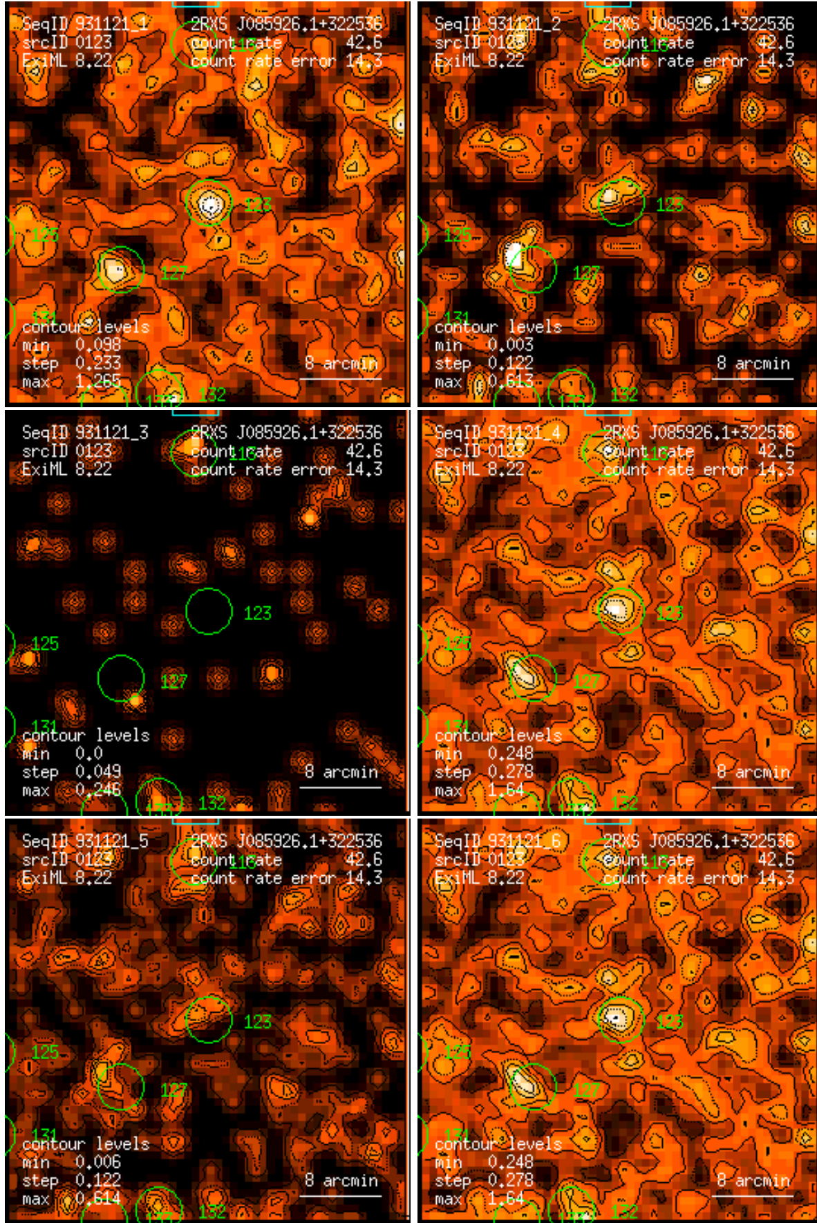
Figure 123: RASS 931121: detection 0123: band rate images, Gaussian filter: (1) PSPC channels 11 – 41, (2) 52 – 90, (3) 91 – 201, (4) 11 – 235, (5) 52 – 201, (6) 11 – 201. Broad band rates in counts/ks. Band rate contour levels in counts/ks/arcmin 2 .
