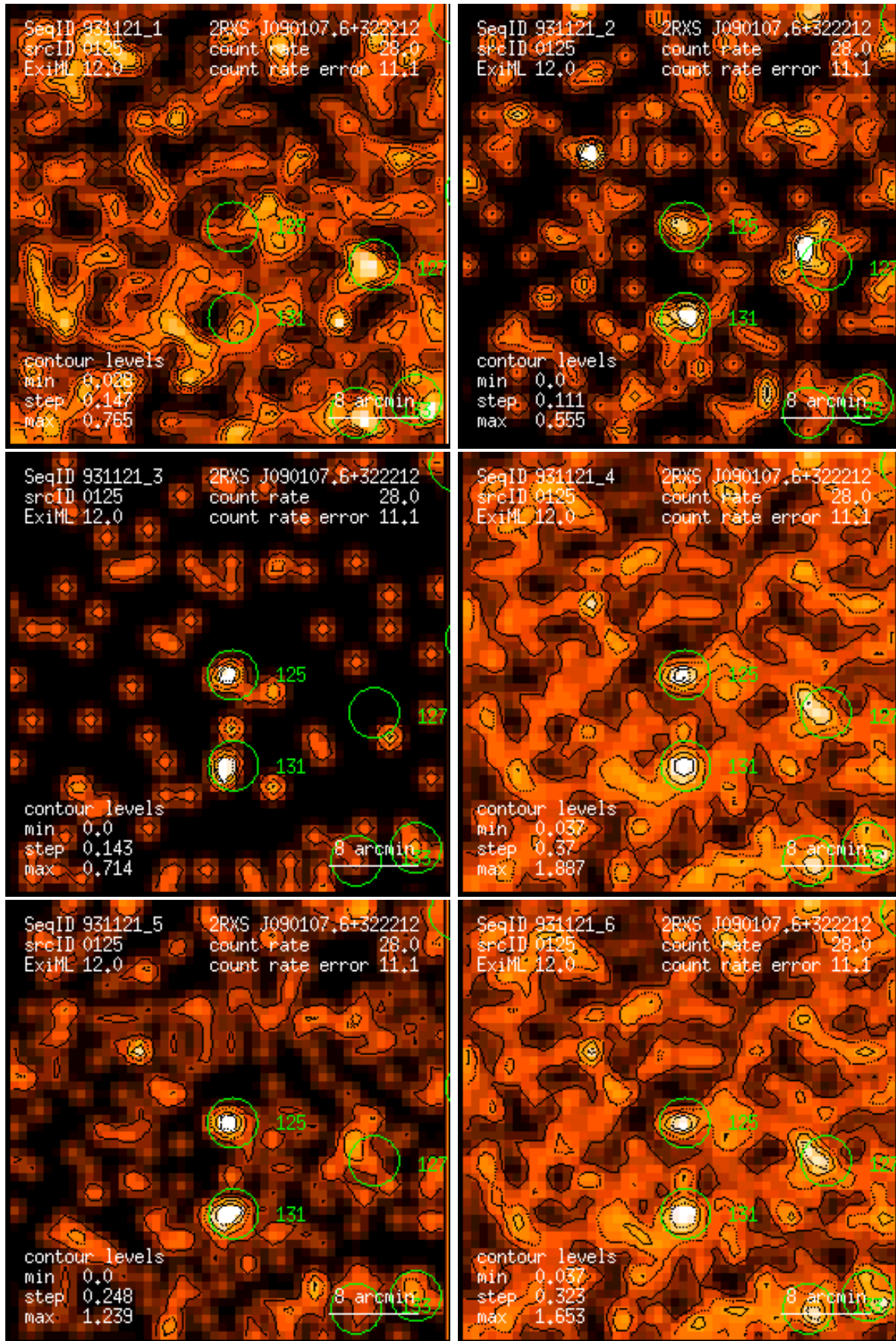
Figure 125: RASS 931121: detection 0125: band rate images, Gaussian filter: (1) PSPC channels 11 – 41, (2) 52 – 90, (3) 91 – 201, (4) 11 – 235, (5) 52 – 201, (6) 11 – 201. Broad band rates in counts/ks. Band rate contour levels in counts/ks/arcmin 2 .
