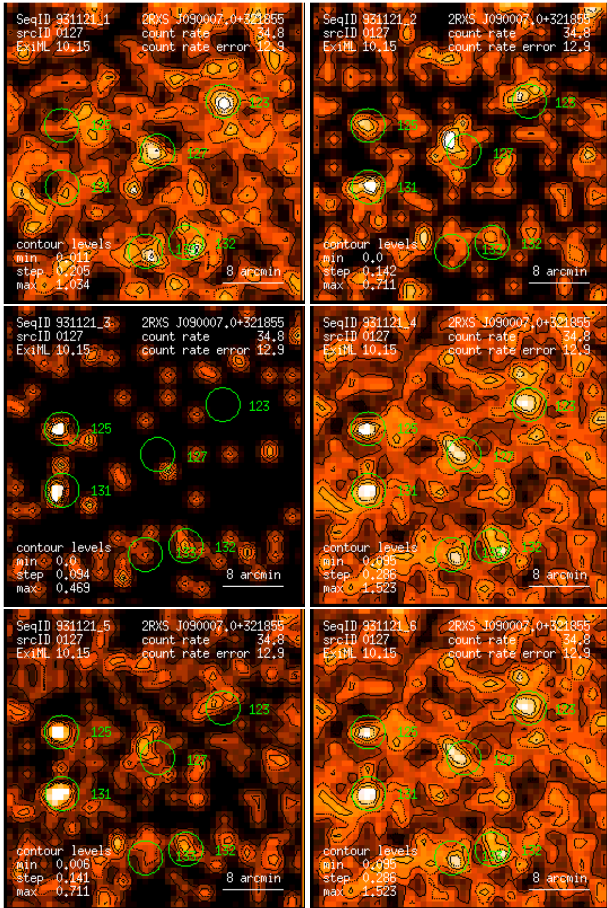
Figure 127: RASS 931121: detection 0127: band rate images, Gaussian filter: (1) PSPC channels 11 – 41, (2) 52 – 90, (3) 91 – 201, (4) 11 – 235, (5) 52 – 201, (6) 11 – 201. Broad band rates in counts/ks. Band rate contour levels in counts/ks/arcmin 2 .
